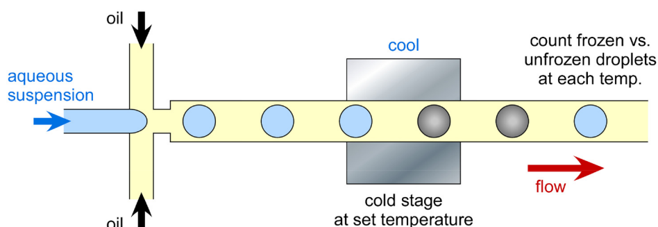
FIG. 7. Continuous flow microfluidic DFAs, in which droplets are generated and then freeze as they pass over a cold stage, allowing the analysis of thousands of droplets. (a) Use of a multi-cold stage instrument to generate a defined temperature gradient. 207 The position at which a droplet freezes thus indicates the temperature at which it froze. (b) Use of a single cold plate, in which the relative number of frozen and unfrozen droplets are counted over a series of set temperatures of the stage, as used in the LOC-NIPI platform. 203 Adapted from Tarn et al. , Lab Chip 20 , 2889–2910 (2020). Copyright 2020, Author(s) licensed under a Creative Commons Attribution 3.0 Unported License.
