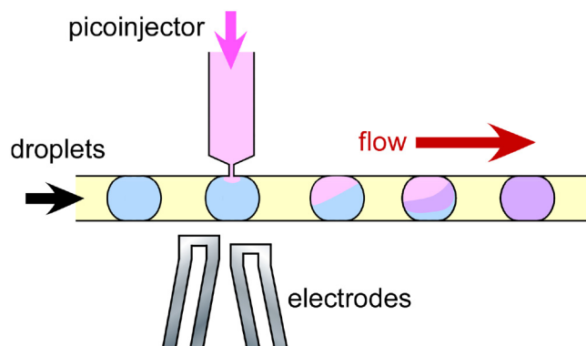
FIG. 9. Pico-injection of biochemical reagents into droplets as they flow past a narrow channel picoinjector. 421 Reprinted (adapted) with permission from Abate et al. , Proc. Natl. Acad. Sci. U. S. A. 107 , 19163–19166 (2010). Copyright 2010 National Academy of Sciences. The interface between the aqueous droplet and the surrounding immiscible oil is momentarily perturbed, allowing injection. The perturbation is often achieved by applying an electric field via microelectrodes, though the use of controlled pressure or the Venturi effect can also be applied. 435 Pico-injection of reagents can allow downstream biochemical analysis to be performed, such as single cell analyses, immunoassays, or DNA analysis.
