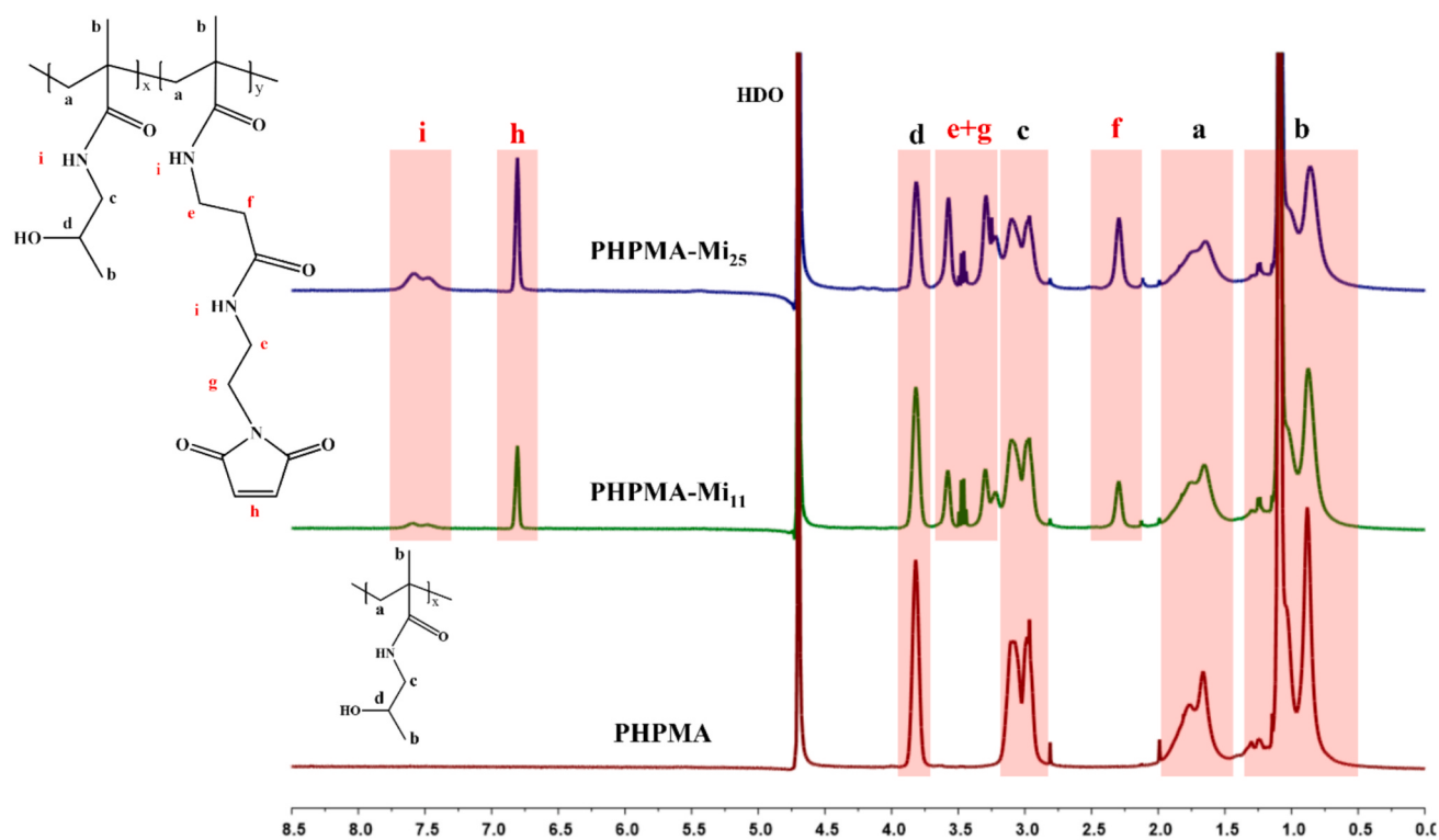
Fig. 2. ^1\text{H} NMR spectra of A – polymer precursors PHPMA-TT recorded in DMSO and B – PHPMA and PHPMA-Mi recorded in \text{D}_2\text{O} .
