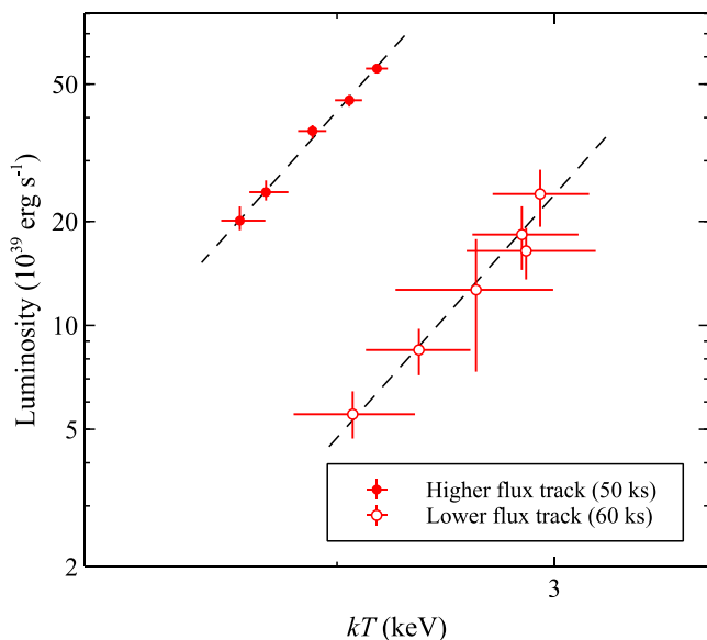
Figure 5. Simulated HEX-P luminosity–temperature constraints for the DISKPB component. For simplicity, we focus only on the magnetic accretor model here, and we also explicitly assume that Holmberg IX X-1 does exhibit two distinct luminosity–temperature tracks that each follow L \propto T^4 when the source has a ‘normal’ hard X-ray flux (i.e. the hard X-ray flux seen in all observations apart from the new soft state discovered here), similar to the results seen from NGC 1313 X-1. In total 11 HEX-P observations are simulated (matching the number of broad-band observations currently in the archive for Holmberg IX X-1), five in the higher flux/lower temperature track (50 ks exposures) and six in the lower flux/higher temperature track (60 ks exposures), with a total exposure of \sim 600 ks. The luminosity–temperature constraints from these HEX-P observations would be either equivalent or superior to the current constraints that combine \sim 1.6 Ms of observing time from XMM-Newton , Suzaku , and NuSTAR .
