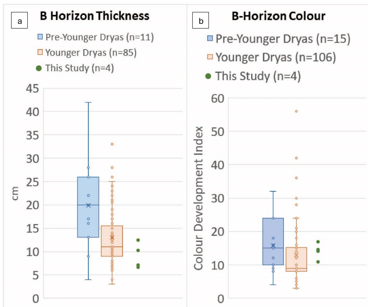
Figure 5.17. Comparison of average B Horizon thickness (a) and colour (b) of Helvellyn sites from this study in comparison with unpublished data from across the Lake District.
