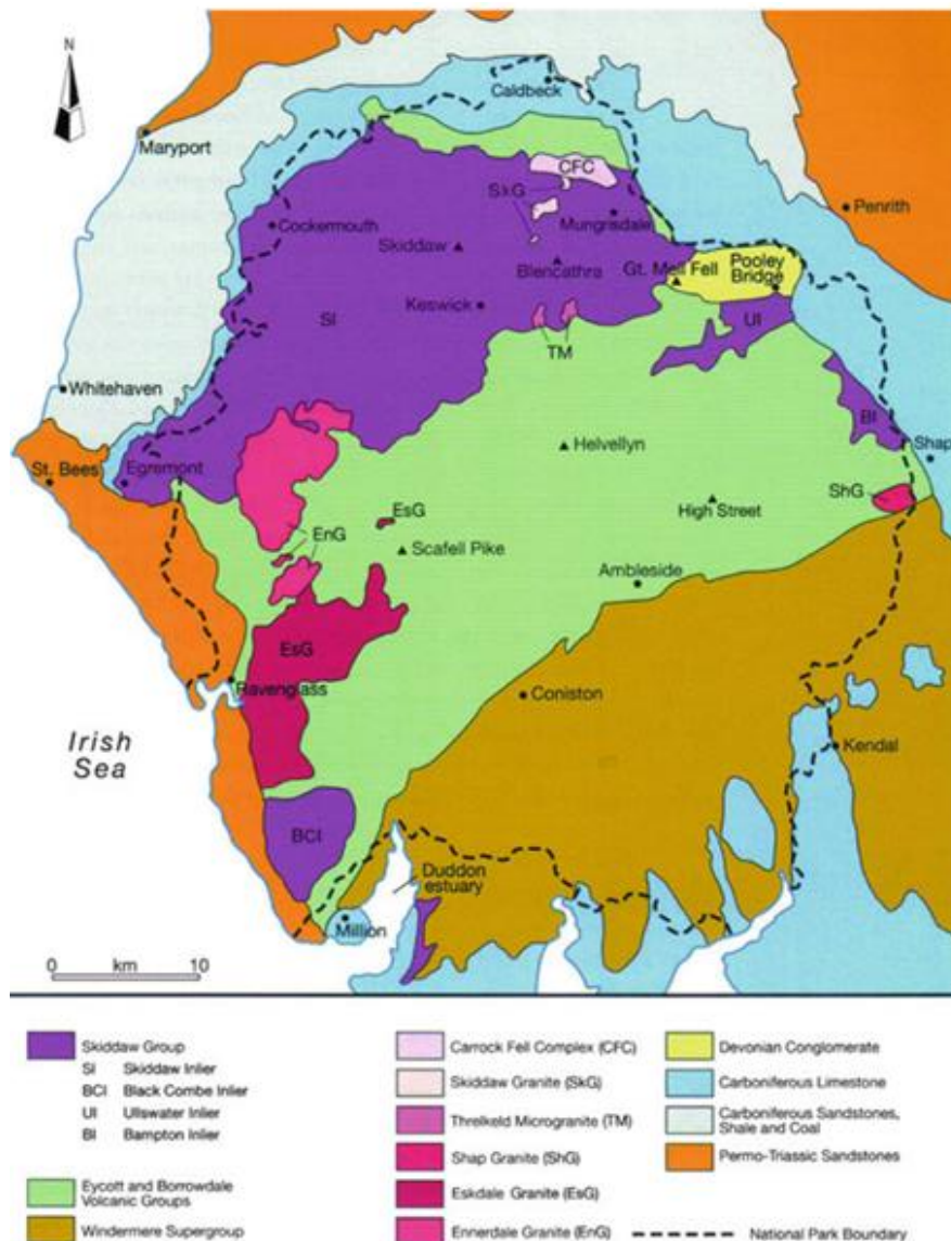
Figure 3.2 Map of the bedrock geology of the Lake District. (From Wilson, 2010)
