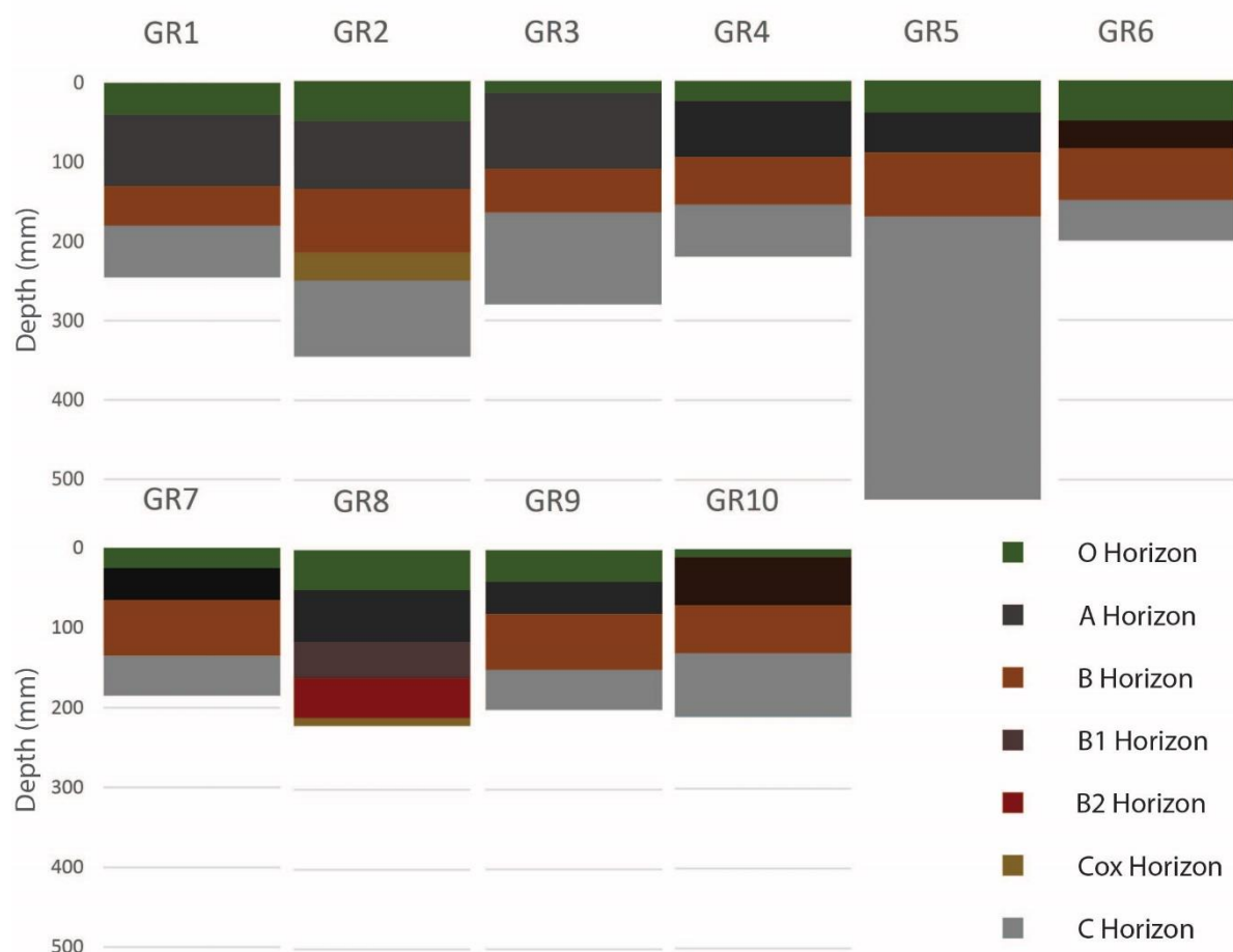
Figure 5.1. Soil horizons observed in Grisedale study sites.
