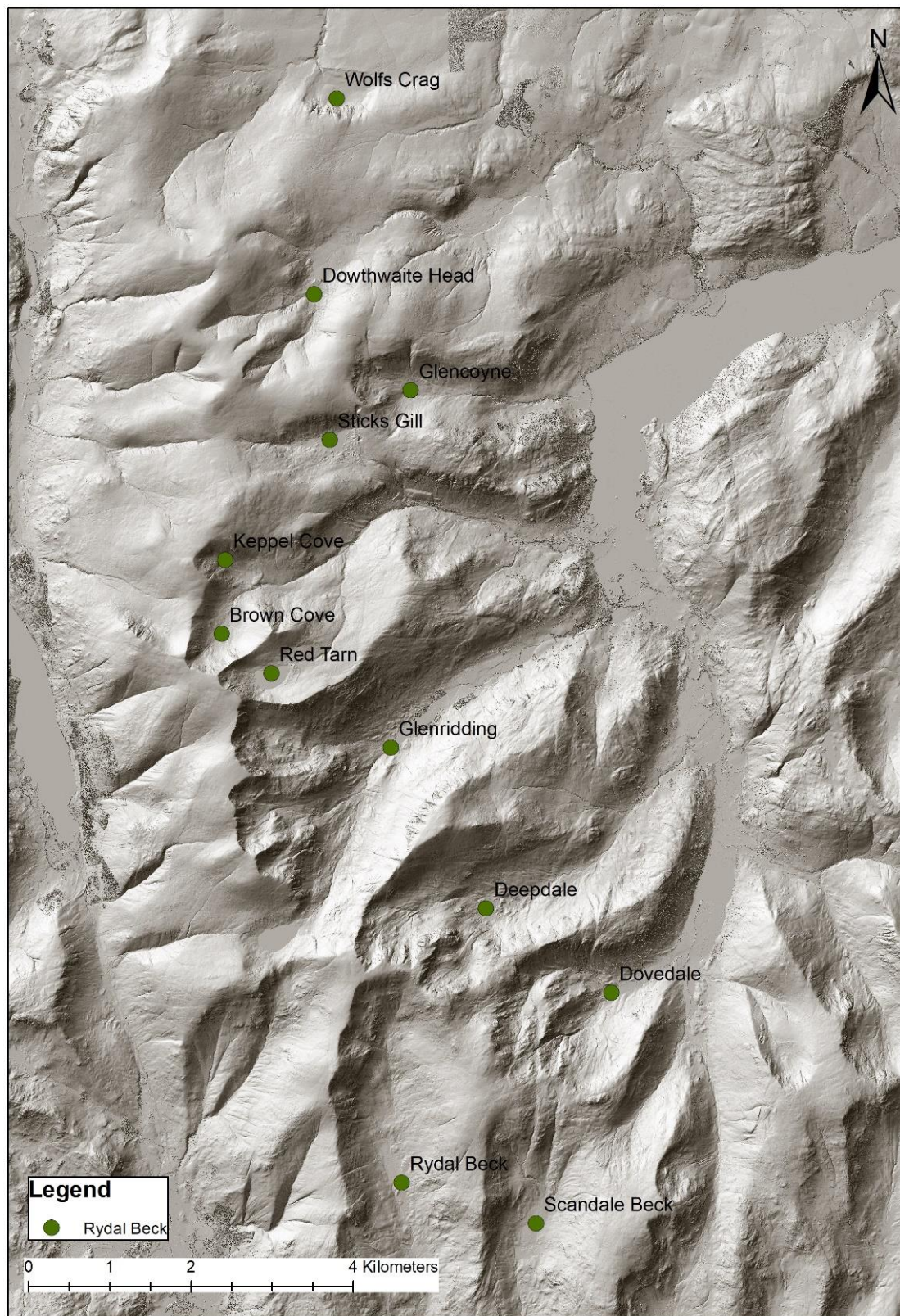
Figure 3.3 Locations of referred to valleys in the Helvellyn range. Basemap is Lidar Composite Digital Terrain Model England 1m resolution © Crown copyright.
