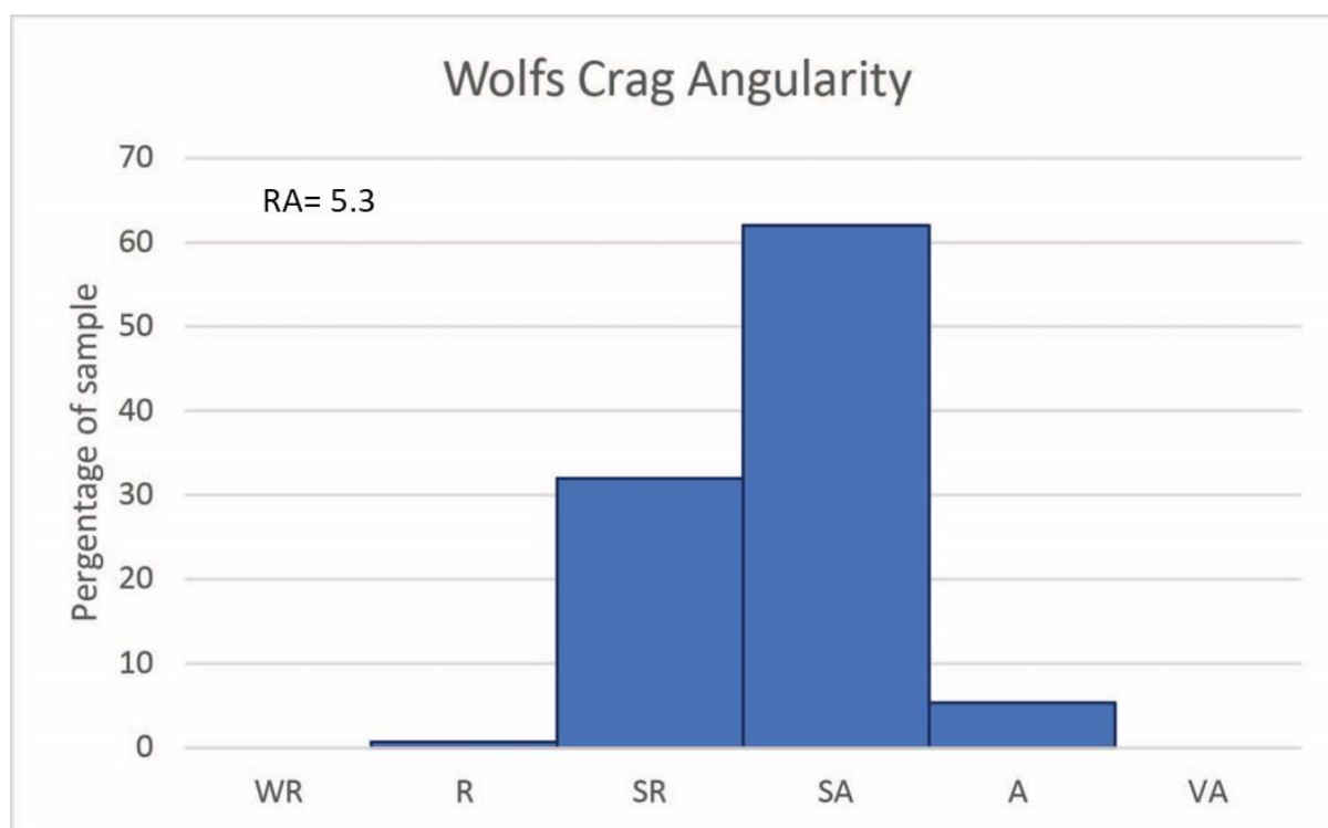
Figure 5.22. Percentage of clasts in Wolfs Crag sample within each of the angularity categories (n=150).
