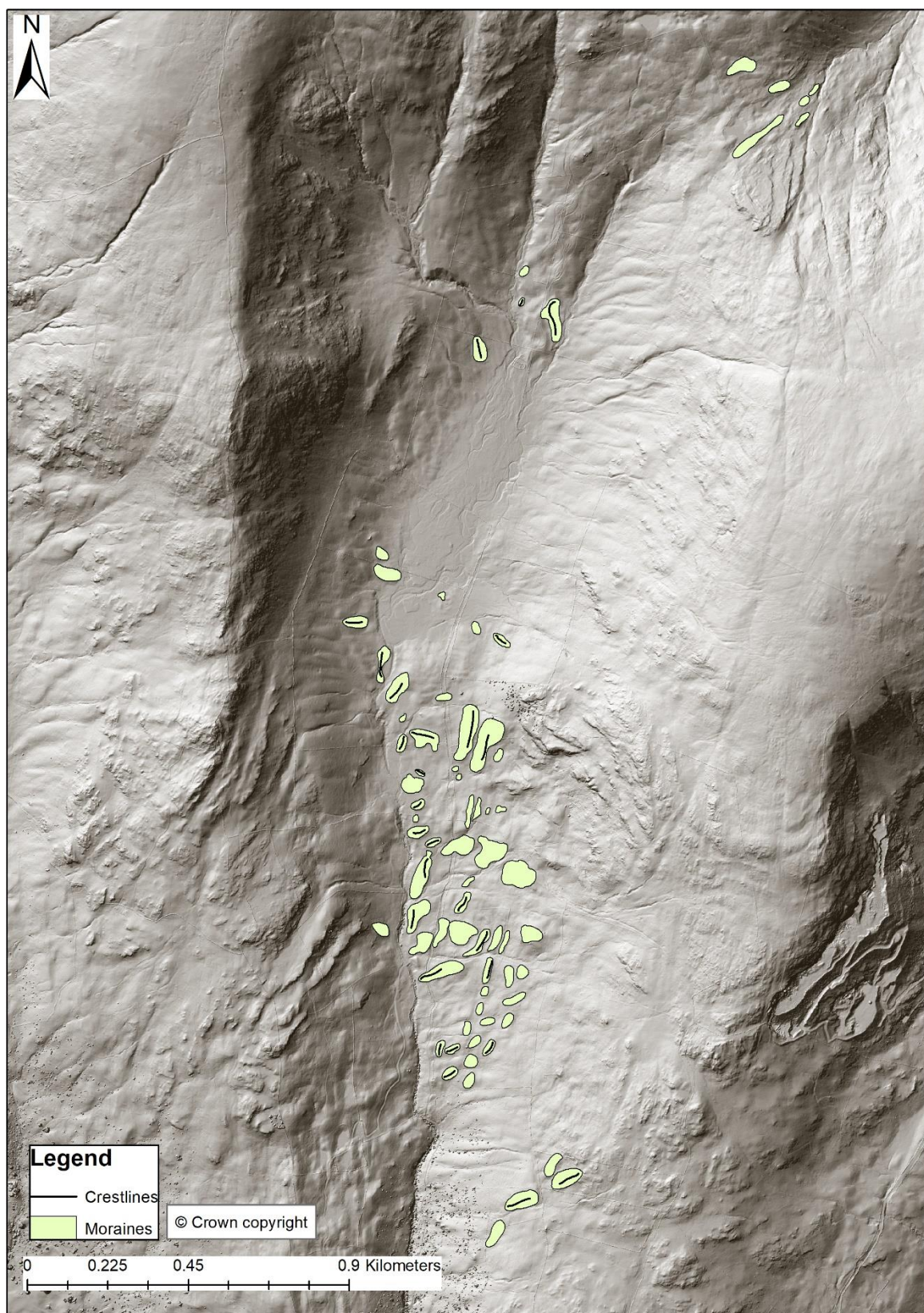
Figure 5.38. Glacial geomorphology of Scandale Beck.
