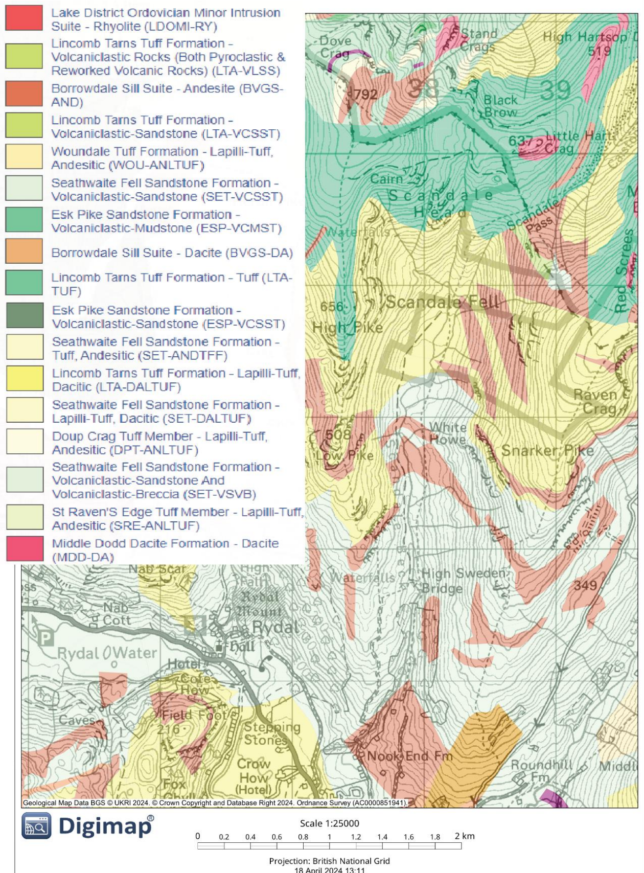
Figure 3.10 9Geological map of Scandale Beck. (Geological Map Data BGS © UKRI 2012)
