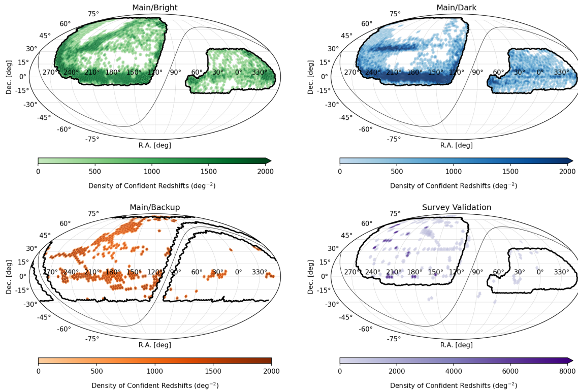
Figure 5. Surface density of all unique targets with good redshifts observed in the bright, dark, and backup main-survey programs (first three panels), and in SV (lower-right panel), rendered using an equal-area Mollweide projection in equatorial coordinates. In each panel, the thin gray curve represents the Galactic plane, which divides the DESI footprint into its north and south Galactic cap regions (shown as thick black outlines; see Figure 3). The density of targets in the bright- and dark-time programs extends to above 2000 \text{ deg}^{-2} , compared to the (as-designed) > 8000 \text{ deg}^{-2} surface density of targets in SV.
