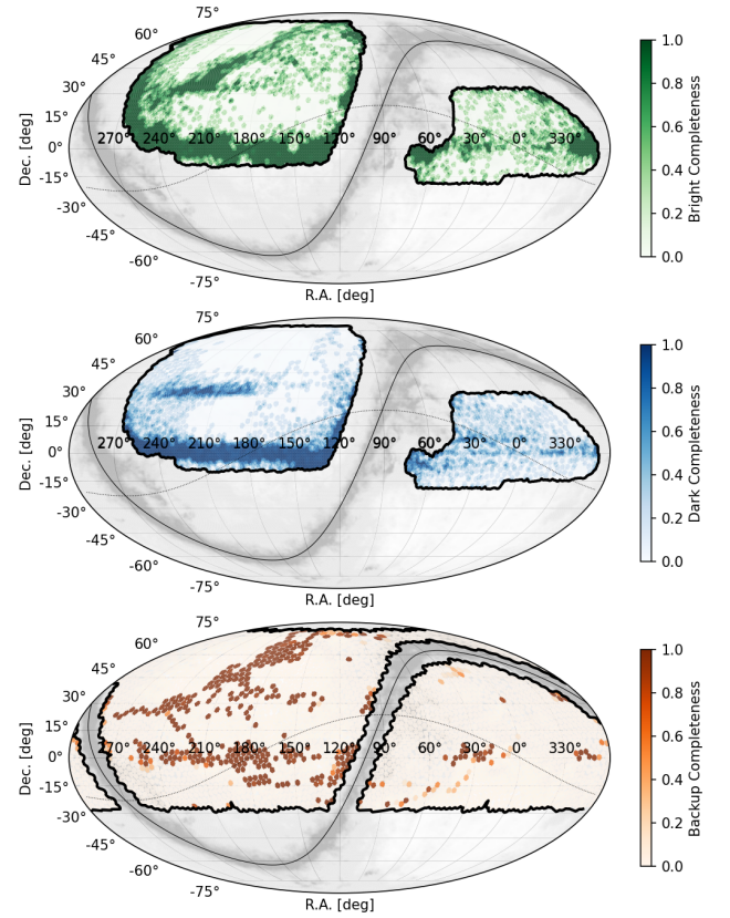
Figure 3. Completeness of the DESI main survey based on observations between 2021 May 14 and 2022 June 13 for the bright, dark, and backup programs (from top to bottom). Dark-shaded areas are complete, while white areas have not yet been observed. We use an equal-area Mollweide projection in equatorial coordinates and indicate the per-program DESI main-survey footprint with a thick black curve. As discussed in Section 2.3.1, the bright- and dark-time footprints are identical, while the backup program footprint extends to lower Galactic latitude. The dashed line shows the Galactic plane, the dotted line shows the ecliptic plane, and we also display the Galactic reddening level outside the DESI footprint in gray.
