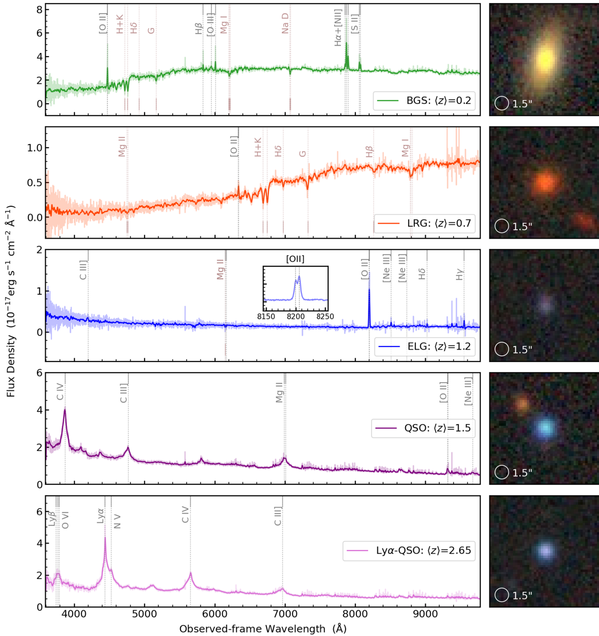
Figure 7. Composite spectra and example LS images of the extragalactic target classes. The left-hand panel of each row shows the average of 75–100 spectra in a narrow redshift slice around the mean redshift value labeled in the lower-right of each panel. For the BGS, LRG, and ELG target classes, we use a bin width of \Delta z/(1+z) = 10^{-5} , and for the QSO and Ly \alpha QSO target classes, we use \Delta z/(1+z) = 3 \times 10^{-5} . The faint colored lines represent the inverse-variance-weighted average spectra, while the darker lines are the same spectra smoothed with a five-pixel Gaussian kernel. The vertical dotted lines indicate the expected wavelengths of key emission and absorption lines, and for the ELG class, the inset shows the resolved [O II] \lambda\lambda 3726, 29 doublet. The right-hand panel of each row features a g, r, z color image of one representative object from each target class, with the fiber diameter of 1.5'' drawn to scale.
