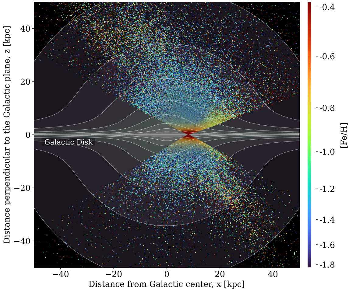
Figure 2. Distribution of Milky Way stars in DESI DR1 observed as part of the MWS. The colors of individual points represent the spectroscopically inferred iron abundance, [\text{Fe}/\text{H}] , as measured using the RVSpecFit pipeline (see Appendix F and S. E. Koposov et al. 2024). The distances to individual stars have been derived using a neural network with stellar parameters as inputs. The thin curves represent the disk stellar mass density contours from the A. M. Price-Whelan (2017) MilkyWayPotential2022 Galactic model. This visualization illustrates the phenomenal size and scale of the DESI stellar survey, the clear negative iron abundance gradient (from the inner disk to the outer stellar halo), as well as the presence of the Sagittarius stream (S. R. Majewski et al. 2003), visible as more orange-tinted points at (x, z) \approx (-10, +40) kpc and (x, z) \approx (20, -20) kpc above and below the Galactic disk, respectively. The map also shows high-metallicity stars extending above the disk at x = 20 kpc caused by the Monoceros “stream” structure (H. J. Newberg et al. 2002; M. Jurić et al. 2008).
