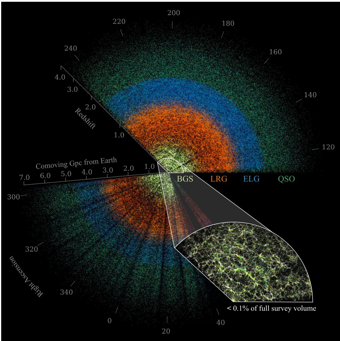
Figure 1. Slice of the Universe mapped by DR1 drawn from a small wedge of the DESI footprint between \pm 5^\circ in decl. out to z \approx 4 . We render the four major extragalactic samples—BGS galaxies, LRGs, ELGs, and QSOs—using yellow, orange, blue, and green points, respectively. Within each target class, the shade of the color maps to decl. (lighter colors correspond to higher decl.). The inset shows a subset of the BGS survey extending out to redshift z = 0.2 , highlighting the LSS traced by galaxies in the densest survey region. For reference, this small wedge of the BGS survey represents less than 0.1% of the comoving cosmological volume in DR1. Also note the black streaks of apparent missing points (most visible at right ascensions between 40^\circ and 300^\circ ), which are due to incomplete survey coverage in DR1, which will be populated in future data releases (see Section 3.2).
