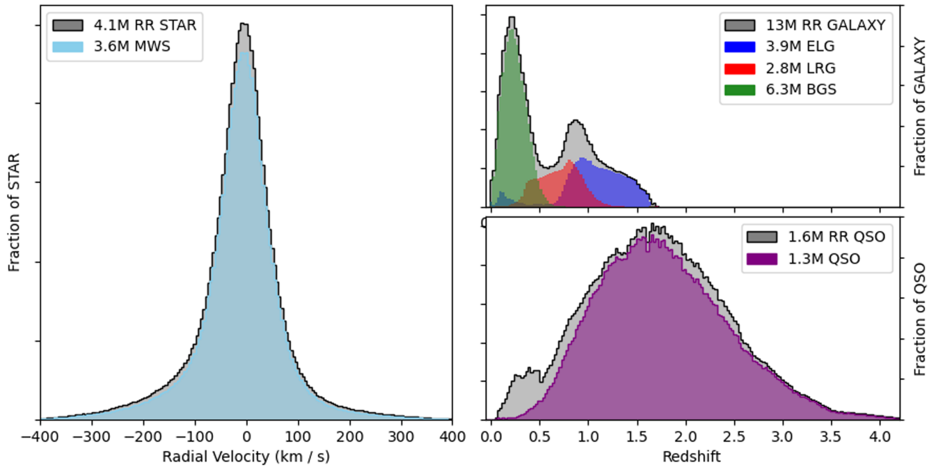
Figure 6. Distribution of objects with confidently measured redshifts in DR1 (see Table 7). In each panel, the gray histograms show objects spectroscopically classified by RR as stars (RR STAR), galaxies (RR GALAXY), or quasars (RR QSO; see Section 3.1.2), the light blue histogram shows the radial velocity distribution of MWS targets, and the dark green, red, dark blue, and purple histograms show the redshift distributions of all unique BGS, LRG, ELG, and QSO DESI targets, respectively. Note that a given object can belong to more than one target class and may therefore appear in more than one distribution.
