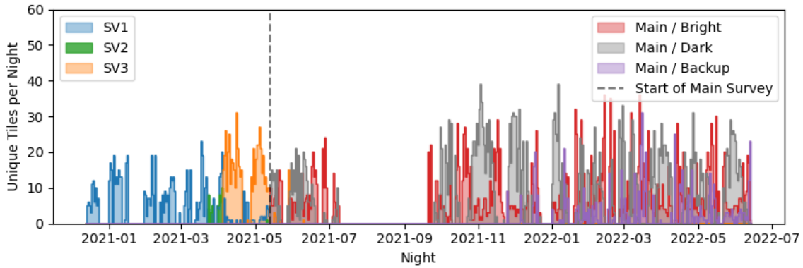
Figure 4. Number of unique SV and main-survey tiles in DR1 as a function of the night (see Table 4). Note that tiles can be observed on multiple nights and that the vertical dashed line indicates the start of the main survey on 2021 May 14. The large gap in observations between 2021 July 10 and 2021 September 20 was due to a major upgrade of the focal-plane electronics.
