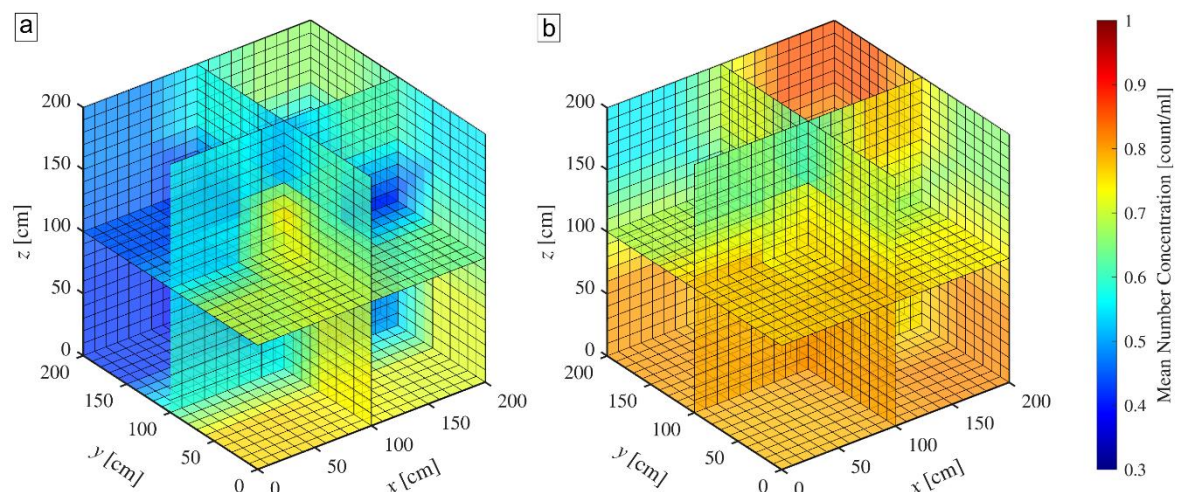
Fig. 2. Slice views of the 10-minute mean particle number concentration field for (a) internal fan switched off and (b) internal fan switched on.
