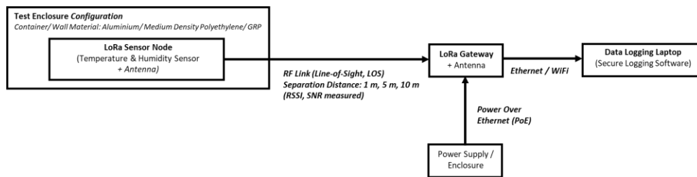
Fig. 1. Schematic representation of the experimental setup showing the LoRa sensor node within the enclosure and the externally positioned gateway under line-of-sight conditions.
