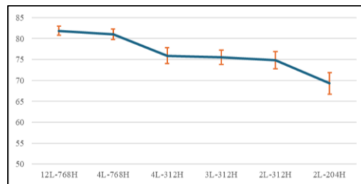
Fig. 2. Comparison of the average performance obtained by different student model configurations.
