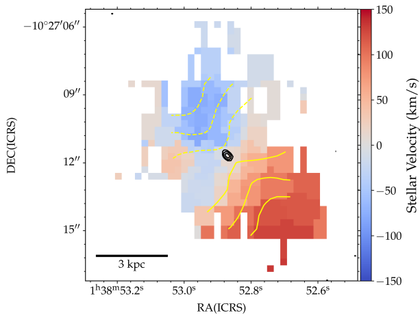
Fig. 8. Line-of-sight stellar velocity map derived from Keck/KCWI BH1L cube using ppxf. Only spaxels with stellar emission stronger than \text{SNR} > 5 (i.e., within the yellow contour in Figure 3) are shown. See Section 3.3 for details. ALMA 334 GHz continuum contours from Figure 2 are shown in black. The velocity field is reproduced by model of a rotating disk at inclination i \sim 60^\circ and position angle \text{PA} \sim 220^\circ , shown in yellow contours, in levels of [40, 70, 90] \text{km s}^{-1} , with blue-shifted velocities shown in dashed lines (see Section 4.1).
