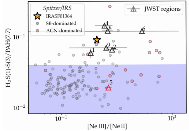
Fig. 16. Ratio between the summed fluxes of \text{H}_2 0\text{--}0 \text{ S}(1) - \text{S}(3) and the 7.7 \mu\text{m} PAH feature, with respect to the [\text{Ne III}]/[\text{Ne II}] line flux ratio. Measurements from regions 1–9 are shown in triangles, and region 5 (the nucleus) is colored in red. Region 3 and 7 are excluded due to poor detection of the 7.7 \mu\text{m} PAH feature. Measurements with Spitzer/IRS for the GOALS sample from Inami et al. (2013) and Stierwalt et al. (2014) are shown in grey circles, with AGN-dominated systems outlined in red. Star marks the Spitzer/IRS measurement for IRAS F01364. The purple shaded area indicate threshold from PDR modeling (Guillard et al. 2012). All extranuclear regions show excess \text{H}_2 emission consistent with previous Spitzer/IRS measurement but the nucleus show low \text{H}_2/\text{PAH} ratio consistent with prediction for PDR.
