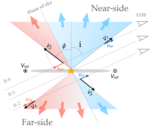
Fig. 15. Schematic of the kinematic model for the biconical outflow observed in IRAS F01364, modified from Heckman et al. (1990) and Veilleux et al. (2001). The three gray dotted lines represent the potential lines-of-sight (LOS) towards regions 8, 5, and 2 (R-8, R-5, R-2) along the bicone, and the plane-of-sky is indicated by the dashed gray line. The yellow star and elongated ellipse respectively represent the nuclear starburst and the surrounding gaseous disk rotating at v_{\text{rot}} , viewed at an inclination angle i . The half opening angle the bicone is given by \phi , and blue-shifted and red-shifted projected velocities are colored in blue and red, respectively. Each component is labeled based on the structure of origin (e.g., NF: near-side cone, front wall; FB: far-side cone, back-wall, etc.). Deprojected velocities are colored black.
