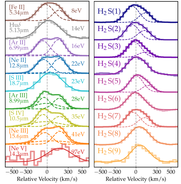
Fig. 4. Spectral profiles of atomic (left) and rotational \text{H}_2 lines (right) detected in the MRS nuclear spectrum, defined in Section 3.1.1 and shown in Figure 2 (in black). All profiles are normalized by the peak line flux density, displayed in velocity space relative to the expected line center based on the redshift of the galaxy (i.e., z = 0.04819 ) and offset vertically for visualization. From top to bottom, the atomic lines are arranged in order of increasing ionizing potential, and the \text{H}_2 lines are ordered from \text{H}_2 0-0 S(1) to \text{H}_2 0-0 S(9). The best-fit models are displayed in solid lines, with individual fitted Gaussian components shown in dashed lines. The best-fit parameters are presented in Table D.1. See Section 3.1.2 for details. Most ionized gas tracers and some \text{H}_2 lines show signs of multiple kinematic components, while broad components with \text{FWHM} > 500 \text{ km s}^{-1} are only detected in the former.
