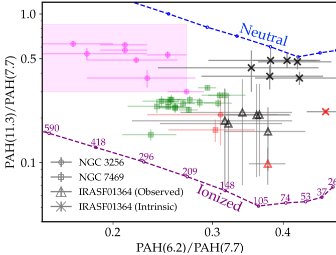
Fig. 11. PAH band ratios measured between the 11.3 and 7.7 \mu\text{m} features with respect to the ones between 6.2 and 7.7 \mu\text{m} features, from region 1–9. Region 3 and 7 are not shown due to poor coverage of the 6.2 and 7.7 \mu\text{m} features. Observed and attenuation-corrected values are shown in triangles and crosses, respectively. Measurements for NGC 7469 from Lai et al. (2022) are shown in squares, and those for NGC 3256 from Bohn et al. (2024) are shown in circles and the pink shaded region. Red-colored symbols mark the AGN. Dashed lines mark the theoretical tracks from Draine et al. (2021) for neutral (blue) and ionized grains (purple) with varying numbers of carbon atoms (indicated in purple texts). Similar to the other two LIRGs, in IRASF01364, the dust grains are more ionized at the AGN than in the extranuclear regions. No clear differences in grain sizes are observed between the AGN and non-AGN regions.
