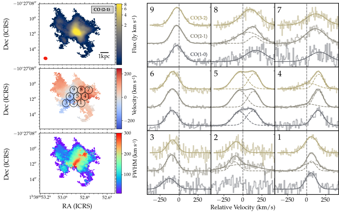
Fig. 7. Spectral analysis of the ALMA datasets. Left: Moment maps of integrated flux, velocity and line width FWHM of the CO ( J = 2-1 ) emission, with the spectral extraction regions defined in Section 3.1.3 (same as in Figure 5) overlaid on the velocity map. The synthesized beam is indicated with a red ellipse in the lower left corner of the flux map. Right: Extracted line profiles of multi- J CO lines. Profiles are normalized by the peak flux density and offset vertically for better visual distinction, with best-fit model and components shown in solid and dashed lines. The cold molecular gas traced by CO (2-1) shows similar morphology and large-scale velocity gradient along E-W direction as the warm molecular gas (Figure 5). Line profiles are sufficiently characterized by a single component across most regions except for in region 5, where all three transitions show consistent, double-peaked profiles.
