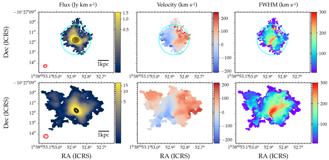
Fig. A.1. Flux, velocity, and line-width FWHM of the CO (J = 1 - 0) and CO (J = 3 - 2) emission, shown in the upper and lower panels, respectively. The 105 GHz and 334 GHz continuum emission in levels of [10, 30, 50] \sigma_{\text{rms}} , and [5, 10, 20] \sigma_{\text{rms}} , are overlaid in black contours over the CO (J = 1 - 0) and CO (J = 3 - 2) flux maps, respectively, where \sigma_{\text{rms}} are reported in Table A.1. Cyan circle mark region C, which encompasses the bulk of the cold molecular gas emission traced by CO (J = 1 - 0).
