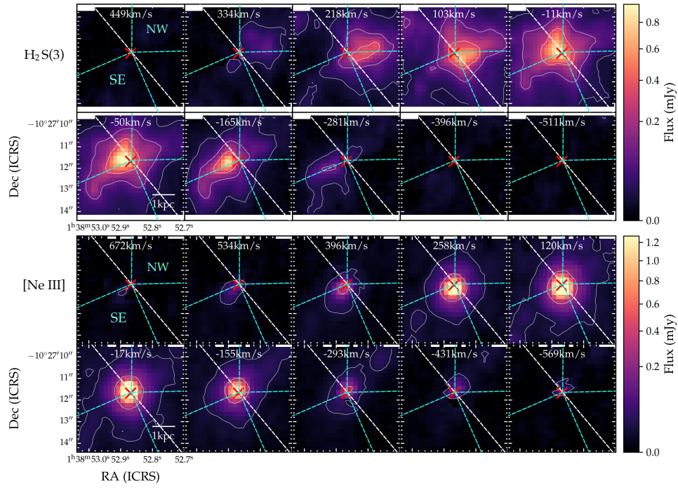
Fig. F.1. Channel maps for (top) \text{H}_2 0-0 S(3) and (bottom) [Ne III] 15.6 \mu\text{m} lines observed with JWST/MIRI-MRS. Red cross mark the position of the nucleus based on the ALMA 334 GHz continuum image. White and cyan dash lines represent the kinematic major axis of the stellar disk, and the outlines of the NW and SE outflow cones, respectively. White contours show levels of 0.015, 0.09, 0.3 mJy, and 0.016, 0.24, 0.8 mJy, for the top and bottom panels respectively.
