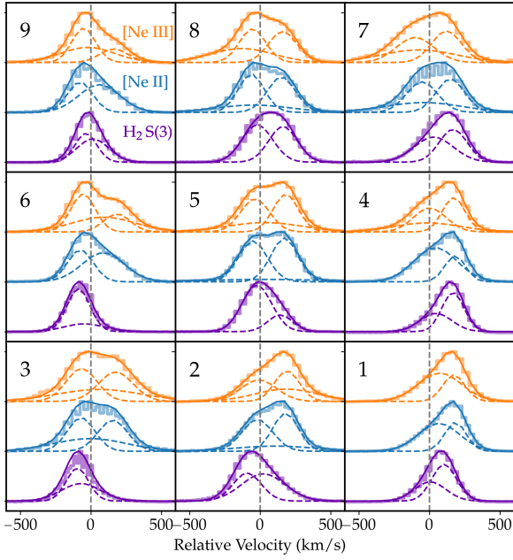
Fig. 6. Line profiles of [Ne III], [Ne II] and \text{H}_2 0-0 S(3) extracted from the nine regions defined in Section 3.1.3 and shown in Figure 5. Profiles are normalized by the peak flux density and offset vertically for better visual distinction, with best-fit model and components shown in solid and dashed lines. Broad wings are seen across most regions in the neon lines but not in \text{H}_2 0-0 S(3), which also has overall narrower profiles.
