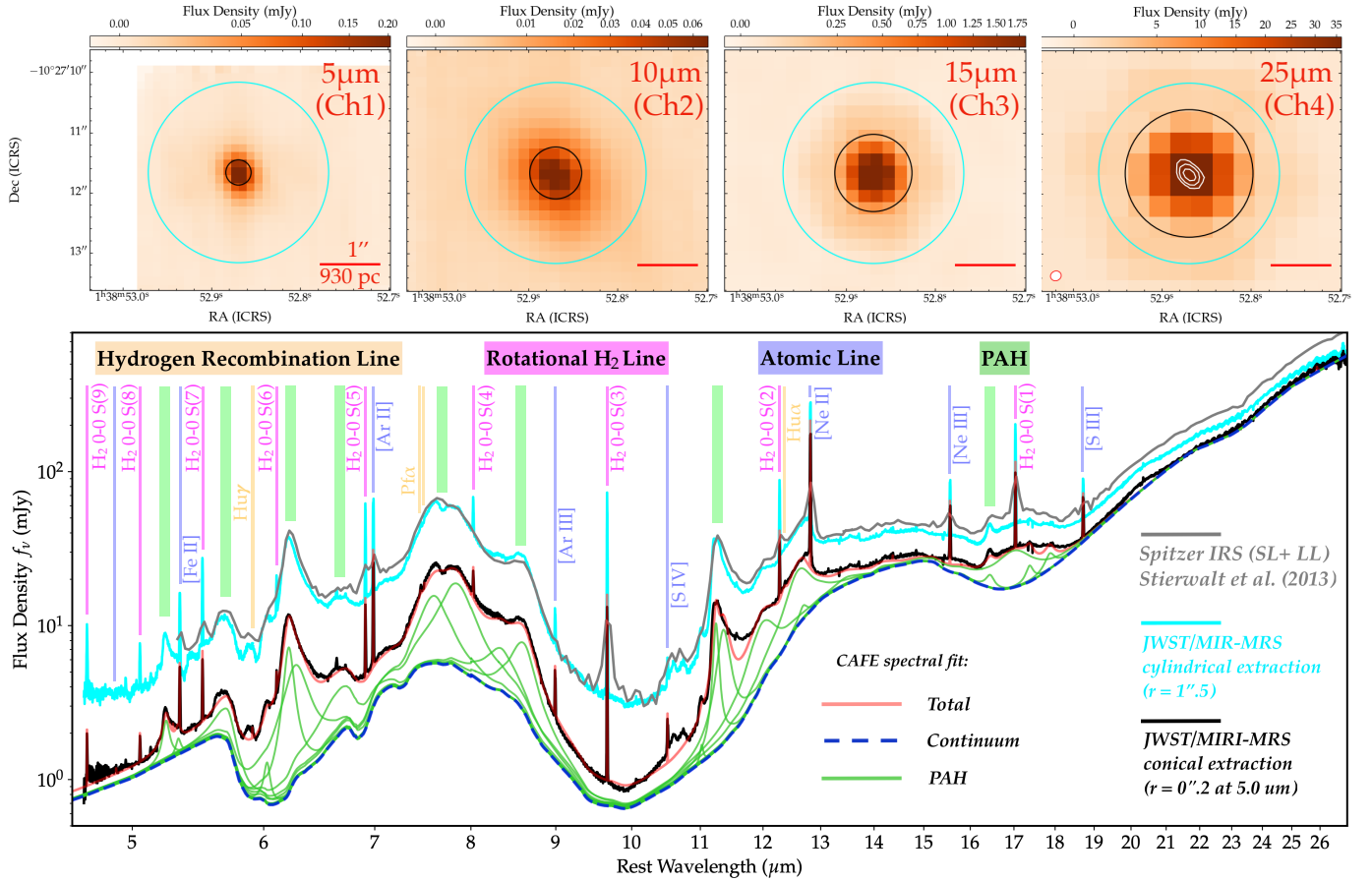
Fig. 2. MIR emission of IRAS F01364 across the MRS wavelength range. Top: Median flux density map at rest-frame 5, 10, 15, 25 \mu\text{m} from ch1, ch2, ch3 and ch4 cubes, respectively. All images are zoomed to the same scale, where the physical size corresponding to 1'' is indicated with the red scale bar in the lower right corner of each panel. The cyan circles, with a fixed radius of r = 1''.5 , indicate the cylindrical aperture used to extract the integrated MIR spectrum from the central \sim 3 kpc of the galaxy that is covered by all channel cubes. The black circles indicate the expanding conical aperture, with r = 0''.2 at 5 \mu\text{m} and r = 1''.0 at 25 \mu\text{m} , used to extract the spectrum of the compact ( \sim 100 pc) nuclear starburst, as portrayed by the ALMA 334 GHz continuum image, shown in white contours. The red ellipse indicates the synthesized beam size of the 334 GHz continuum image (see Section 2.3). Bottom: Spitzer/IRS spectrum from Stierwalt et al. (2013) (in grey), compared to the full MRS spectra extracted with the fixed-radius, cylindrical aperture (cyan) and expanding conical aperture (black). For the latter, the total fitted spectral profile and the underlying continuum and PAH profiles from CAFE spectral decomposition are overlaid in red, dark blue (dashed) and green, respectively. See Section 3.1 for details. While recovering the emission previously detected with Spitzer/IRS, the high spectral resolution of MRS allows a much more detailed characterization of the various MIR emission and absorption features present in IRAS F01364.
