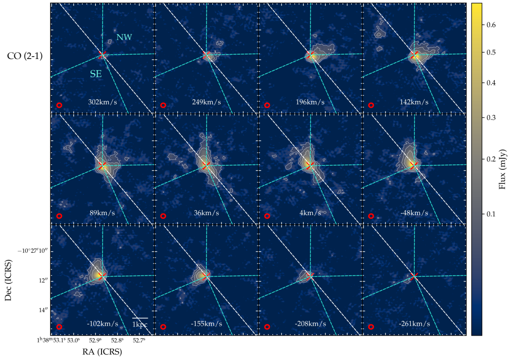
Fig. F.2. Channel maps for the CO ( J = 2 - 1 ) line observed with ALMA. Red cross, white and cyan dashed lines are the same as in Figure F.1. White contours show levels of 0.04, 0.07, 0.14 mJy.
