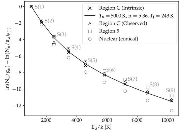
Fig. 14. H _2 excitation diagram and best-fit result assuming a continuous power-law temperature model as prescribed in Togi & Smith (2016), with an upper temperature limit set to 5000\text{ K} . Measurements from region C (Figure 9) are shown in triangles and crosses, for observed and extinction-corrected values, respectively. Extinction-corrected measurements from the nuclear region (Figure 2) and region 5 (Figure 2) are shown in empty gray circles and squares, respectively. Extinction correction mostly affects the measurement of the H _2 0-0 S(3) line. Compared to region C, region 5 shows somewhat higher contribution from S(6) – S(9) lines, while the nuclear (conical) region shows much lower contribution from S(3) – S(9) lines, indicating that the warmer molecular gas components are concentrated at the nucleus.
