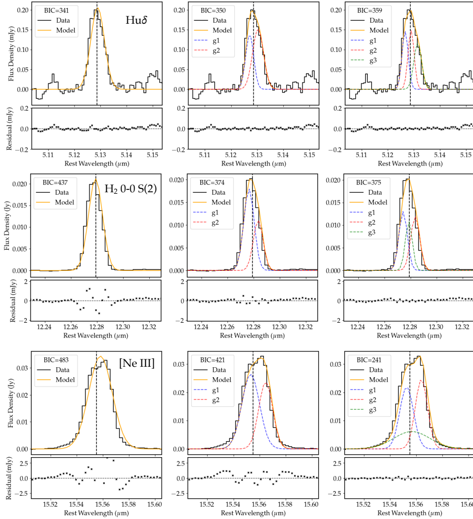
Fig. C.1. Continuum-subtracted line profiles of the \text{Hu}\delta , \text{H}_2 0-0 S(2), and [\text{Ne III}] lines detected in the nuclear MRS spectrum (Figure 2), shown in black curves, respectively in the top, middle and bottom panels. The model fitting results (in orange curves) and residual using one, two and three Gaussian components are shown from left to right. The individual Gaussian components (i.e., “g1”, “g2”, “g3”) for multi-Gaussian models are shown in dashed blue, red and green curves.
