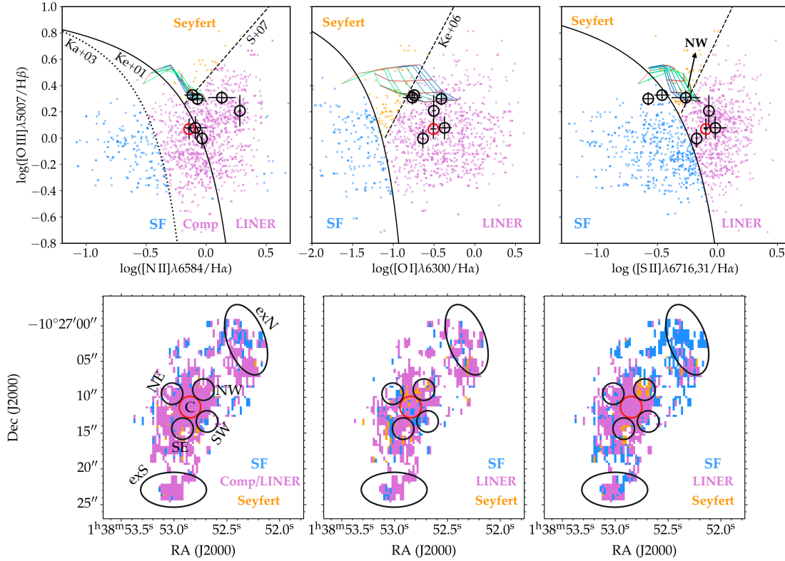
Fig. 13. Classification of the excitation mechanisms of the ionized gas in IRASF01364 based on the optical BPT diagrams (Baldwin et al. 1981; Veilleux & Osterbrock 1987) using \log ([\text{O III}]\lambda 5007/\text{H}\beta) vs. \log ([\text{N II}]\lambda 6584/\text{H}\alpha) , \log ([\text{O III}]\lambda 5007/\text{H}\beta) vs. \log ([\text{O I}]\lambda 6300/\text{H}\alpha) , \log ([\text{O III}]\lambda 5007/\text{H}\beta) vs. \log ([\text{S II}]\lambda 6716,31/\text{H}\alpha) , from left to right, respectively. Top: measured line ratios at each spaxel are shown in blue, purple and orange, for classifications of “star formation”, “composite/LINER”, “Seyfert” excitation, respectively. The demarcation lines are defined by Kauffmann et al. (2003) (Ka+03), Kewley et al. (2001) (Ke+01), Schawinski et al. (2007) (S+07), and Kewley et al. (2006) (Ke+06). Model grids for fast radiative shock with the same parameters as in Figure 12 are overlaid. Bottom: spatial distribution of spaxels with different classifications. In all panels, circles mark measurements/locations of the regions defined in Section 3.3, with region C highlighted in red. Most optical line emission in the IRASF01364 can be attributed to composite/LINER excitation. Region NW shows Seyfert-like line ratios in the [\text{S II}]/\text{H}\alpha diagram, which may be due to AGN photo-ionization or shocks.
