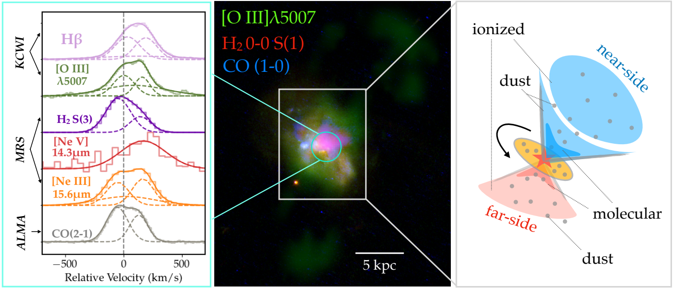
Fig. 10. Multiphase gas morphology and kinematics derived from Keck/KCWI, JWST/MIRI-MRS, and ALMA data. Left: Comparison of line profiles of emission lines detected in the multiwavelength datasets in the central 3 kpc in region C, defined in Section 3.1.1 (see also Figure 2). Profiles are normalized by the peak flux density and offset vertically for better visual distinction, with best-fit model and components shown in solid and dashed lines. Middle: Color-composite overlay of ALMA CO (1-0), MRS H 2 0-0 S(1) and Keck/KCWI [O III] λ5007 emission on top of the F336W/F435W/F814W tri-color HST image from Figure 1, showcasing the multiphase biconical structure emerging from the dust-obscured nucleus of IRASF01364. The cyan ellipses highlight the regions defined in Section 3.3 for analyzing the large-scale ionized gas emission. Right: Simplified representation of the molecular and ionized outflow bicones with respect to the stellar disk (in yellow ellipse) and the nucleus (red star). The black curved arrow indicates the rotation of the stellar disk inferred from Figure 8. The cold and warm molecular gas are co-spatial and trace the inner edges of the ionized bicone, and appear brighter and more extended on the near-side NW cone.
