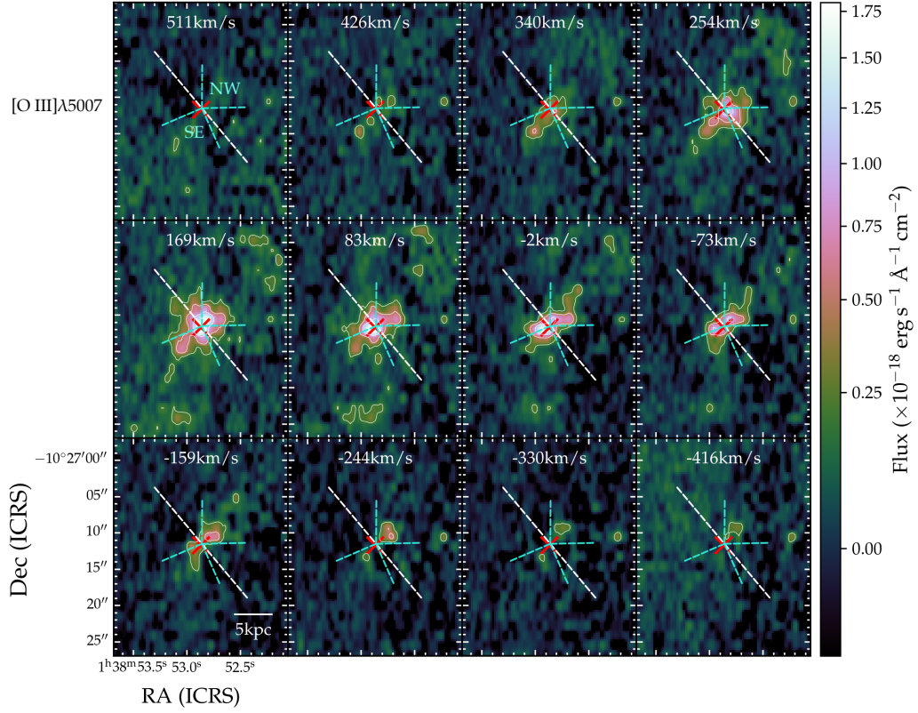
Fig. F.3. Channel maps for the [\text{O III}]\lambda 5007 line observed with Keck/KCWI. Red cross, white and cyan dashed lines are the same as in Figure F.1. White contours show levels of 0.2, 0.5, 1.0 \times 10^{-18} \text{ erg s}^{-1} \text{ \AA}^{-1} \text{ cm}^{-2} .
