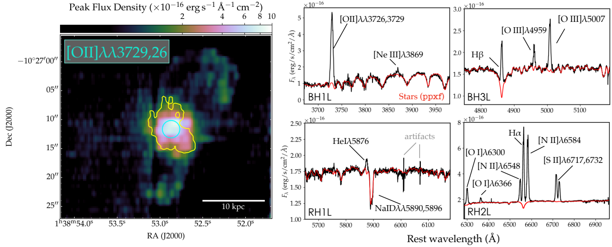
Fig. 3. Optical emission of IRASF01364 as observed by Keck/KCWI. Left: Map of the peak flux density of the [O II] \lambda\lambda 3729,3726 line, overlaid with the 5\sigma contour of the stellar continuum measured in the adjacent wavelength range, in yellow. For context, the cyan circle marks the aperture used to extract the integrated MRS spectrum shown in Figure 2. The same aperture is used to extract the spectra shown in the right panels. Right: KCWI spectra extracted from the final reduced and aligned BH1L, BH3L, RH1L and RH2L cubes. The fitted stellar spectra derived from ppxf are shown in red. See Section 3.3 for details. The [O II] emission map reveals extended ionized gas emission around IRASF01364 beyond the bulk of the stellar emission on 10 kpc-scale. A number of other key emission lines are also detected, allowing further characterization of the ionized gas properties.
