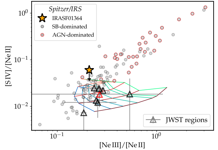
Fig. 12. [\text{S IV}]/[\text{Ne II}] vs. [\text{Ne III}]/[\text{Ne II}] ratios across region 1–9, shown in triangles. Region 5 (the nucleus) is colored in red. Region 7 is not shown due to poor detection of the [\text{S IV}] 10 \mu\text{m} line. Measurements with Spitzer/IRS for the GOALS sample from Inami et al. (2013) are shown in grey circles, with AGN-dominated systems outlined in red. The star marks the Spitzer/IRS measurement for IRASF01364, where only an upper limit for [\text{S IV}]/[\text{Ne II}] was obtained. Model grids for fast radiative shock with solar metallicity and pre-shock electron density of 100\text{ cm}^{-3} (Allen et al. 2008; Sutherland et al. 2018) are overlaid in colored lines, with orange-brown lines representing shock velocities from 100\text{--}200\text{ km s}^{-1} and blue-green lines representing magnetic field strengths from 1\text{--}100\text{ }\mu\text{G} . All regions show line ratios similar to starburst-dominated systems, which are also consistent with the range predicted by models of fast radiative shock.
