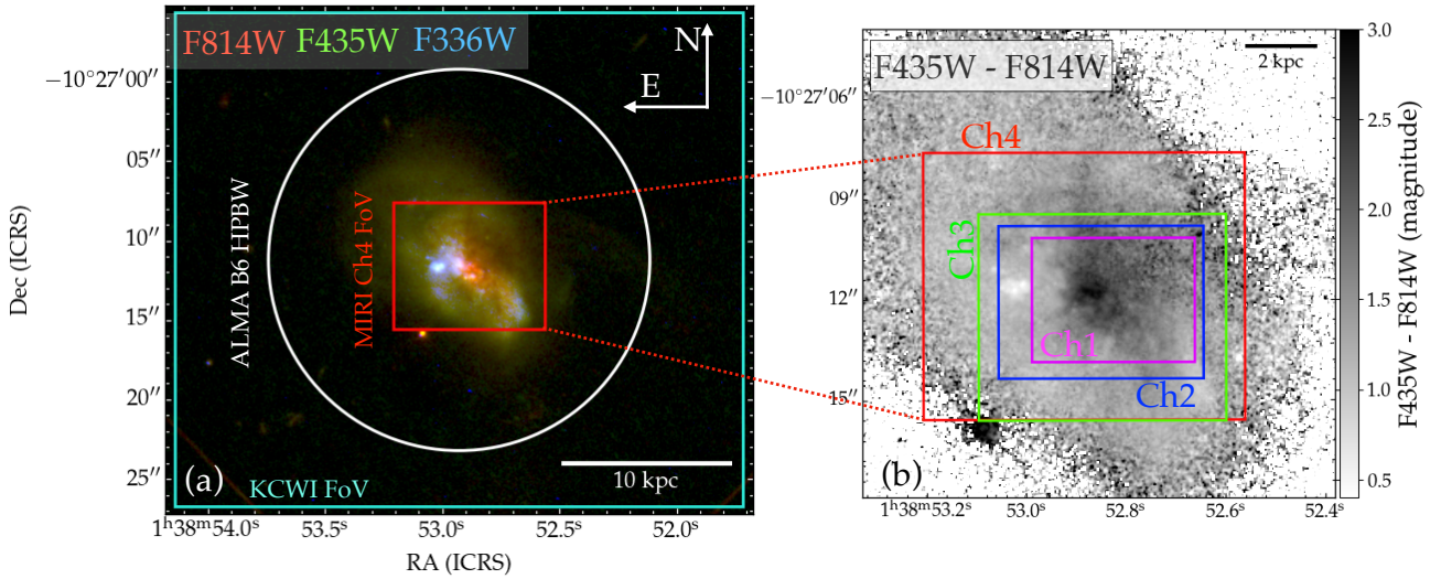
Fig. 1. HST images of IRAS F01364-1042. (a) False color image with F336W, F435W and F814W filters, which are represented in blue, green and red, respectively. The Half-Power-Beam-Width (HPBW) of the ALMA Band 6 primary beam, and the fields-of-view (FoVs) of the calibrated data cubes from Keck/KCWI and the longest wavelength channel of JWST/MIRI-MRS (i.e., ch4) are outlined in white, cyan, and red, respectively. (b) Zoom-in on the HST F435W – F814W map in magnitude, where a darker grey shade indicates a redder (F435W – F814W) color, and thus higher dust extinction. Colored boxes outline the FoVs of the JWST/MIRI-MRS ch1-ch4 cubes. Prominent, nonuniform dust structures can be seen extending from the nucleus out to \sim 5 kpc into the galaxy. The large FoVs of the Keck/KCWI and ALMA datasets allow characterization of the ISM across the entire system, while JWST/MIRI-MRS probes the immediate vicinity of the dust-obscured nucleus.
