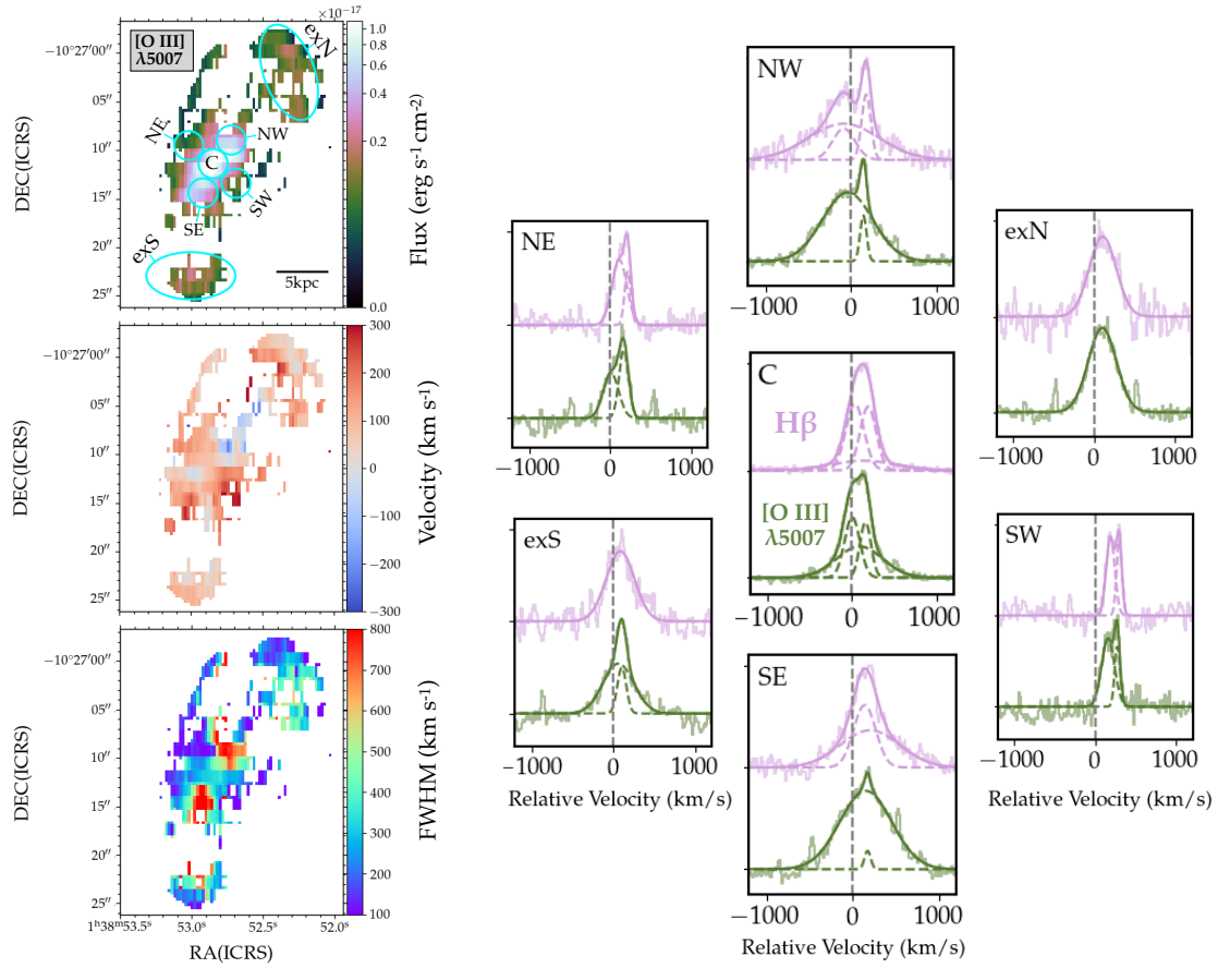
Fig. 9. Spectral analysis of the Keck/KCWI datasets. Left: Maps of integrated flux, velocity, and line-width FWHM of [O III]λ5007 emission, with the spectral extraction regions defined in Section 3.3 overlaid on the integrated flux map. Right: Extracted line profiles of H \beta and [O III]λ5007, normalized by the peak flux density and offset vertically for better visual distinction, with best-fit model and components shown in solid and dashed lines. The ionized gas as traced by [O III]λ5007 extends beyond \sim 10 kpc from the nucleus along the SE-NW direction, with no clear sign of rotation in the central region as seen in the stellar kinematics (Figure 9). Line profiles of both H \beta and [O III]λ5007 exhibit broad wings along the SE-NW direction, i.e., kinematic minor axis of the central stellar disk.
