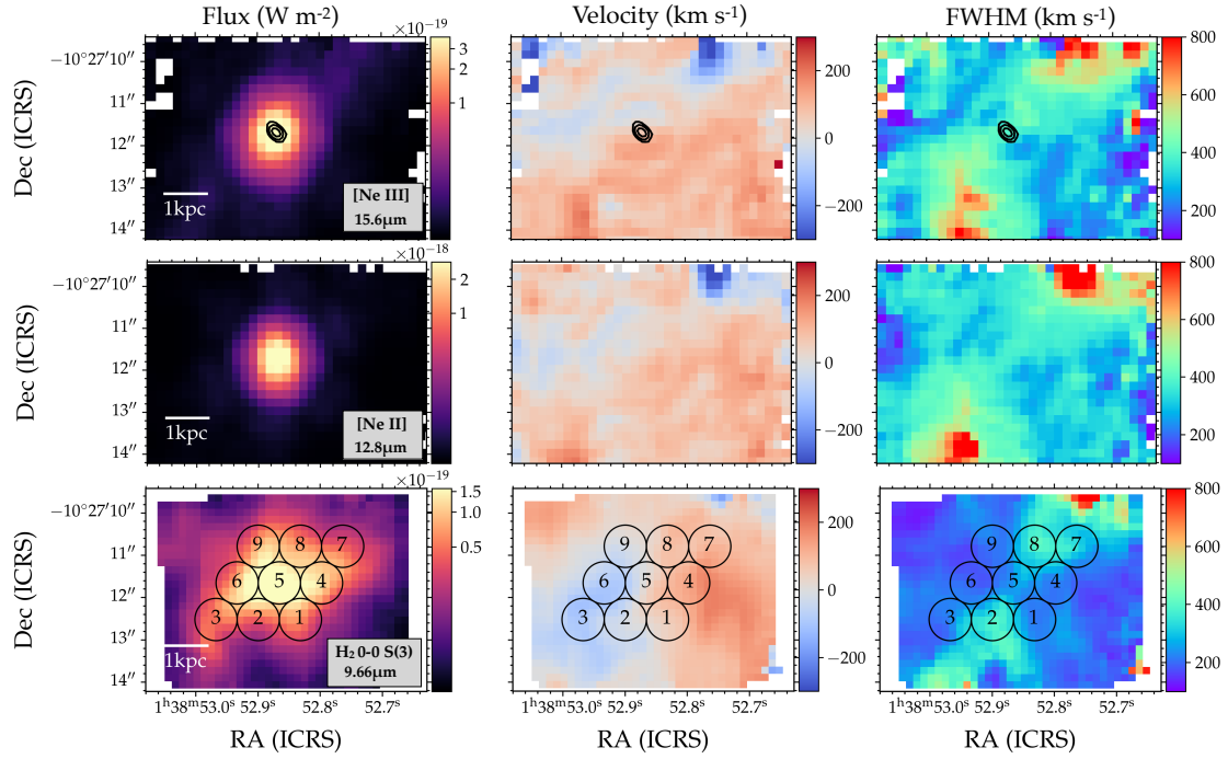
Fig. 5. MRS maps of the integrated line flux, velocity, and FWHM line width for [Ne III], [Ne II], and H 2 0-0 S(3) lines (see Section 3.1.3). Spaxels with SNR < 3 in each line are masked. ALMA 334 GHz continuum contours from Figure 2 are overlaid in the [Ne III] maps, and the spectral extraction regions defined in Section 3.1.3 are overlaid on the H 2 0-0 S(3) maps. While ionized gas tracers ([Ne II], [Ne III]) show compact emission at the nucleus, molecular gas traced by the H 2 line shows extended X-shaped morphology on ~3 kpc scales. Ionized and molecular gas both show enhanced gas dispersion along the SE-NW direction.
