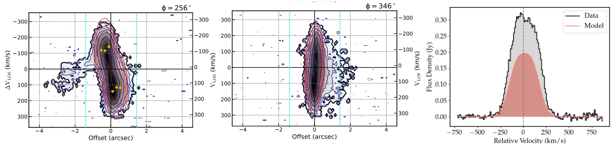
Fig. E.1. modeling results of the central kpc of the CO ( J = 2 - 1 ) emission from 3\text{D} Barolo. The left and middle panels show the PV diagrams of the fitted model of the nuclear rotating molecular disk (in red contours), along the major ( \phi = 256^\circ ) and minor axis ( \phi = 346^\circ ) previously determined by Agostino et al. (2026). The observed emission are shown in grey scales, and area covered by region C is indicated with vertical dashed cyan lines. The right panel compares the observed and modeled CO ( J = 2 - 1 ) line profile extracted from region C, shown in grey and red, respectively. The modeled nuclear disk contributes 60% of the total flux contained within region C.
