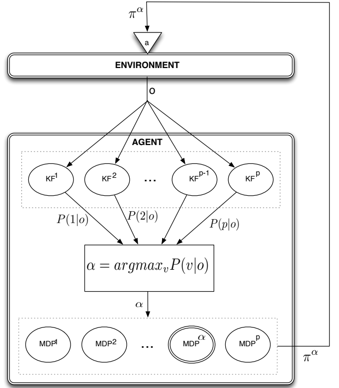
Fig. 1. Architecture overview.
