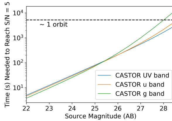
Fig. 16 Point-source sensitivity (AB mag) in each of CASTOR’s three primary passbands, expressed as the time needed to reach a signal-to-noise ratio of S/N = 5 . The time for CASTOR to complete a single orbit is shown as the dashed horizontal line. This calculation assumes the default telescope and detector parameters for CASTOR given in Table 1 of Cheng et al., 17 with the inclusion of Earthshine, zodiacal light, and “average” [O II] 2471 Å geocoronal emission as defined in Sec. 3.2 of the same text and was carried out using version 1.3.2 of the FORECASTOR ETC. The code to generate this curve can be found at https://github.com/CASTOR-telescope/ETC_notebooks/blob/master/snr_table.ipynb .
