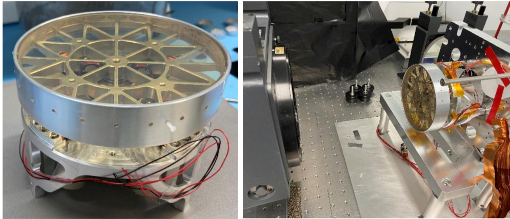
Fig. 4 Zerodur fine steering mirror (FSM) prototype, without reflective coating, undergoing wavefront error testing at the ABB Measurement and Analytics facility in Quebec City. The fully functional FSM tip-tilt mechanism is mounted on a damped optical table, in front of a Zygo interferometer. See Sec. 2.3 for details.
