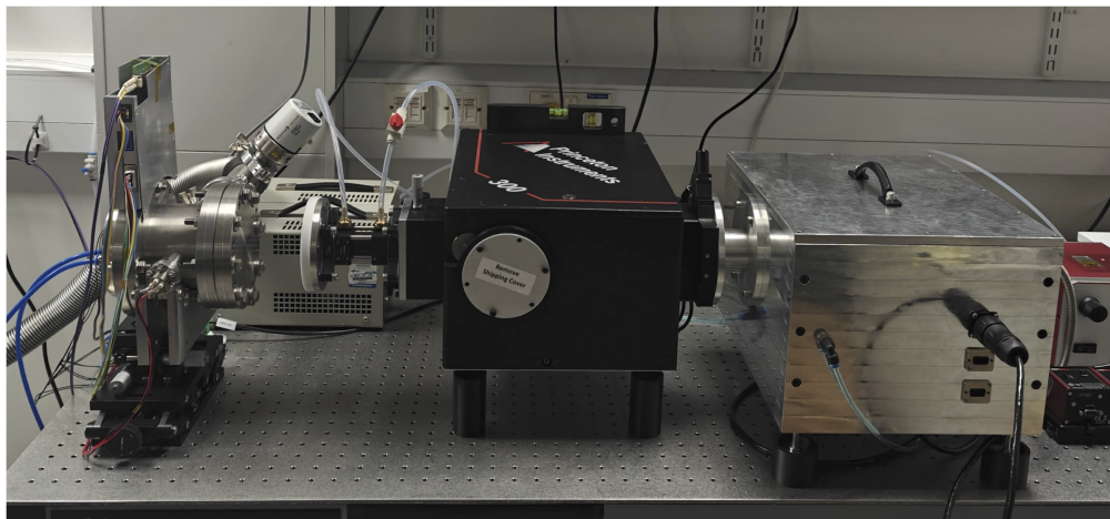
Fig. 22 CIS120 and monochromator test setup at The Open University. A CIS120 device is mounted inside the vacuum chamber on the left, currently set up for dark tests. The chamber on the right is a housing for a dual deuterium and halogen lamp feeding the monochromator in the middle.
