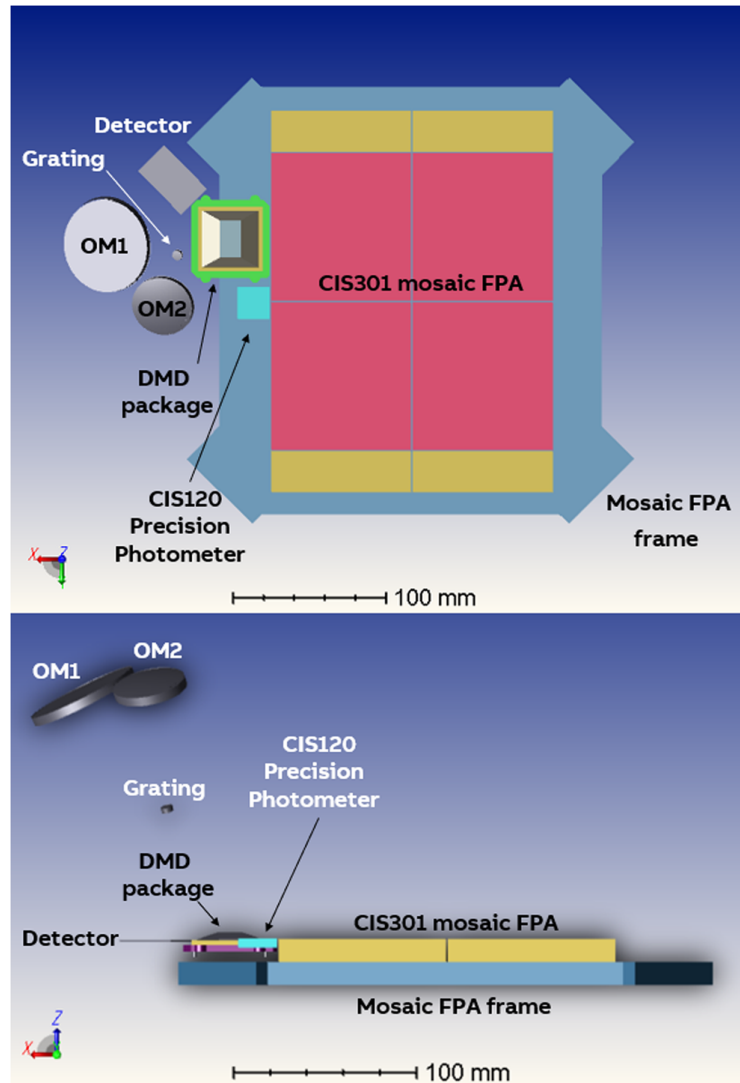
Fig. 23 Front and side view of the UVMOS optomechanical concept (upper and lower panels, respectively). OM1 and OM2 refer to the first and second Offner mirrors.
