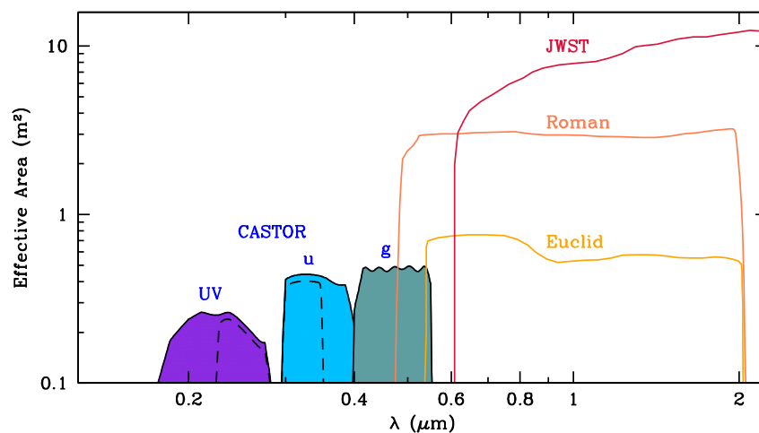
Fig. 2 Effective area as a function of wavelength for current and upcoming UVOIR space telescopes. Each of these facilities provides images having high angular resolution (e.g., FWHM \lesssim 0.2'' ). CASTOR will thus complement red-optical/IR imaging from JWST, Euclid, and Roman. Its wide-field imager uses dichroics to provide simultaneous three-band imaging over the 0.15 to 0.55 \mu\text{m} wavelength range. A deployable broadband filter allows users to subdivide the UV and u channels (dashed curves).
