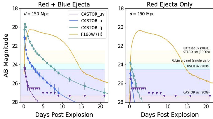
Fig. 10 Mock CASTOR observations of a GW170817-like kilonovae at 150 Mpc using our baseline survey strategy described below. (Left). Expected observations for a transient with both a red (heavy r-process elements) and a blue (light r-process elements) ejecta component. (Right). Expected observations for a transient with only a red ejecta component. Although the infrared emission (yellow curve) is almost unchanged, dramatic differences are evident in the ultraviolet and blue bands on a timescale of 1 to 10 days. Even at these moderate distances, tracing the evolution of the UV emission requires depths of >25 to 26 mag AB. Quoted depths of various proposed UV/ u -band survey missions are highlighted (with depth indicated at the upper boundary of each shaded region).
