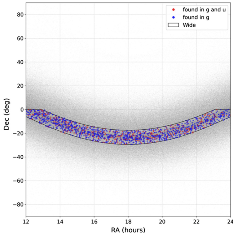
Fig. 15 Simulations of the TNO wide survey component from a high-precision model of the outer Solar System. 73 The wide footprint will include all objects within 6 deg of the ecliptic and having \delta < 0 deg, the region that will be best sampled by LSST. Colored points show the objects detected by the wide component of the CASTOR census of TNOs. Red symbols show objects are detected in both u and g ; blue symbols show objects detected in g only. For clarity, the figure shows only 10% of total model and detected objects and only the 12 to 24 h zone, the part of the ecliptic south of the equatorial plane.
