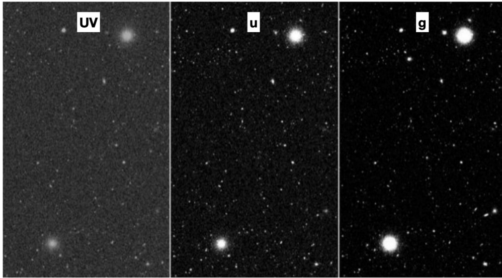
Fig. 19 Simulated images for a small patch of CASTOR's planned Wide Survey in the UV, u , and g channels, generated using a synthetic light-cone catalog drawn from published semi-analytic models of galaxy populations. 78,79 With total exposure times in the range of 1000 to 2000 s, these images reach 5\sigma point-source depths of \sim 27.5 in all three channels.
