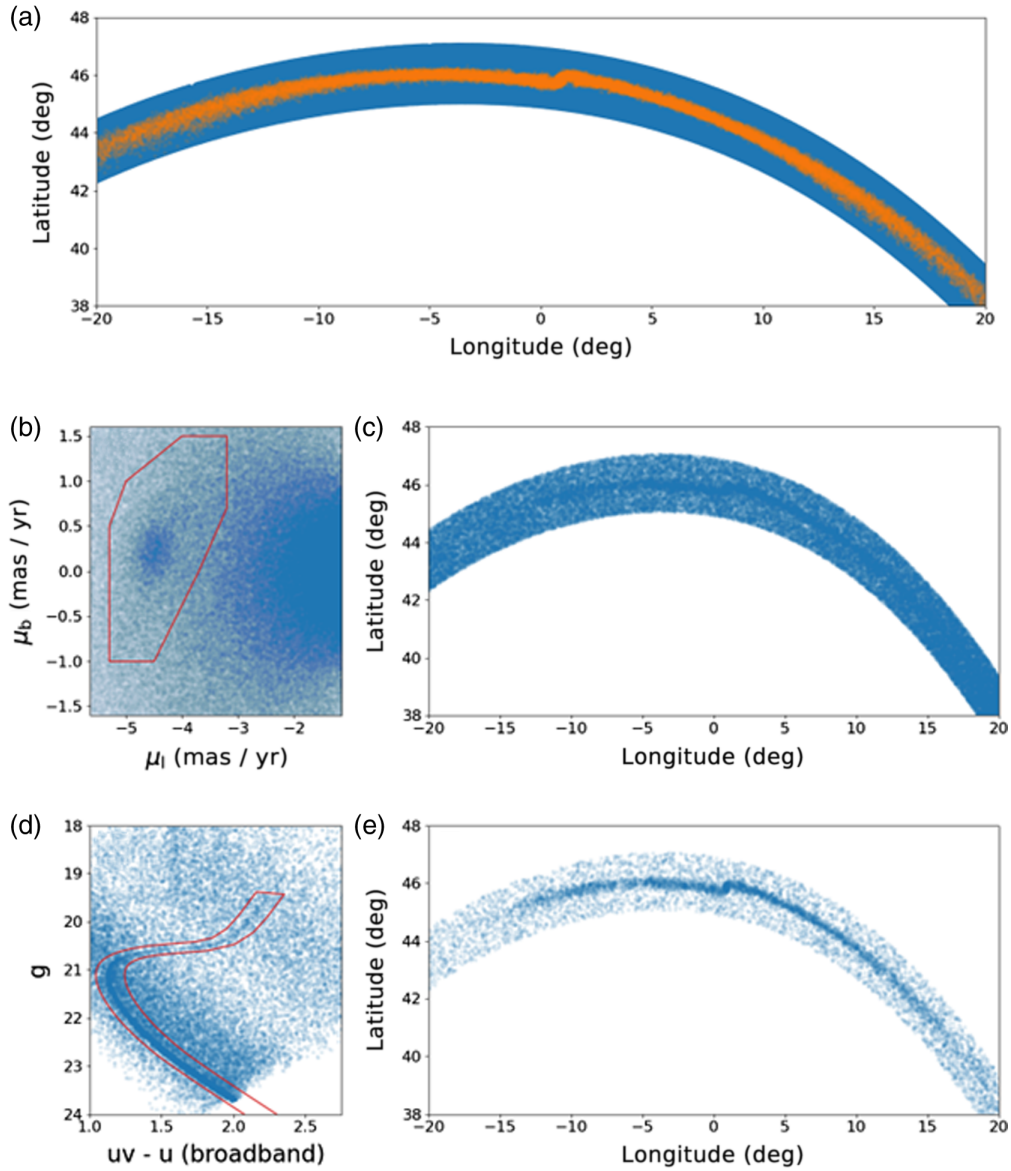
Fig. 13 Mock CASTOR observations of the Pal 5 stellar stream (at a distance of 20 kpc) based on an N-body simulation of the stream (orange points in top panel) inside a smooth Milky Way halo (D. Erkal, private communication) combined with background/foreground contamination from Galaxia 56 stellar catalogs in fields surrounding the stream (blue points). On-sky positions of the stars are shown in the top and right panels. Panel C shows a selection based on the CASTOR proper motions (from panel B). A further selection based on the CASTOR color-magnitude diagram (from panel D; along the metal-poor isochrone corresponding to the stream) is shown in panel E, where the stream appears as a clear overdensity. CASTOR's deeper observations (compared with Gaia ) with a transverse velocity proper motion precision corresponding to 50 km/s or better at this distance (fainter stars with poorer proper motion precision are not included in this figure) will significantly increase the number of stream members identified, improve the contrast, and reveal an unprecedented view of stellar streams and their morphology. The proper motion uncertainties ( <0.5 mas/yr for stars brighter than g \sim 25 ) were calculated assuming a time baseline of 4 years and an exposure time of 2200 s per epoch for each CASTOR field (see Sec. 4.3 of Cheng et al. 17 for more details on the astrometric error budget and proper motion estimates).
