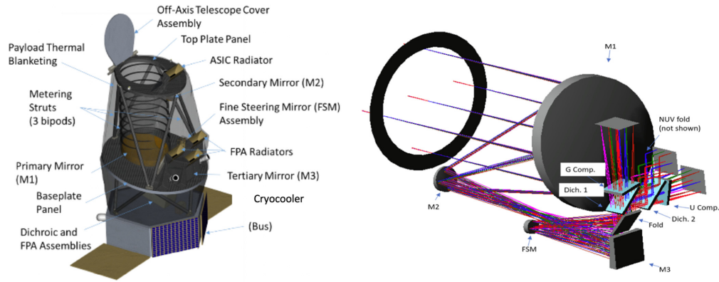
Fig. 3 (Left) Illustration of the main payload elements for the telescope (see Secs. 2.1, 2.2, and 2.5 for details). (Right) Schematic diagram showing the opto-mechanical design of the telescope. An off-axis, three-mirror anastigmat design uses a fine steering mirror for image stabilization and two dichroics to direct the incoming light onto three focal plane arrays (FPAs).
