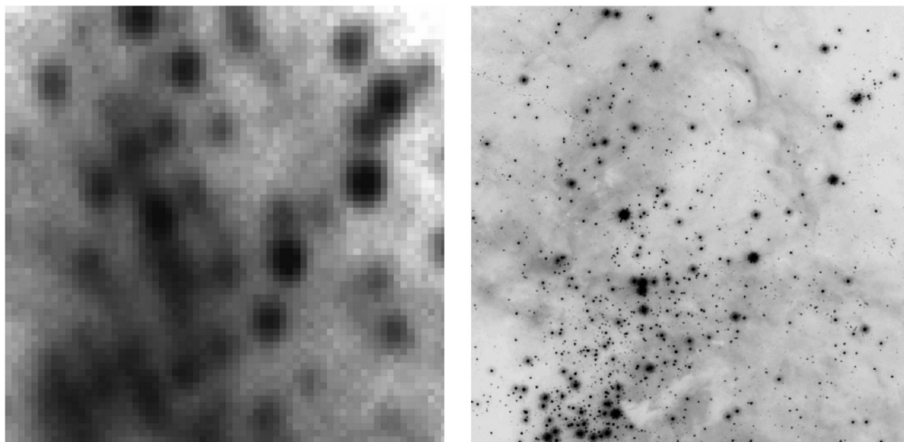
Fig. 14 Observations of a 100'' \times 100'' region in 30 Doradus from GALEX/NUV (left) and simulated CASTOR observations (right) based on smoothed data from HST/WFC3 F275W. The depth is 24 mag, so the CASTOR Magellanic Clouds survey will reach about 50 times deeper.
