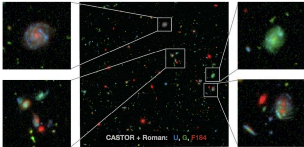
Fig. 12 Simulation of part of the Hubble Ultra Deep Field (UDF) in passbands from CASTOR ( u , g ) and Roman (F184). This image shows a \sim 1.5' \times 1.5' field or just \sim 0.06\% of the area that will be covered by the proposed Ultra-Deep Survey. Although Roman's IR imaging (red) is sensitive to existing stellar mass, CASTOR picks out regions of ongoing star formation. With comparable spatial resolution from the UV to the near-IR, it will be possible to map stellar populations and other physical parameters across galaxies, out to cosmic noon.
