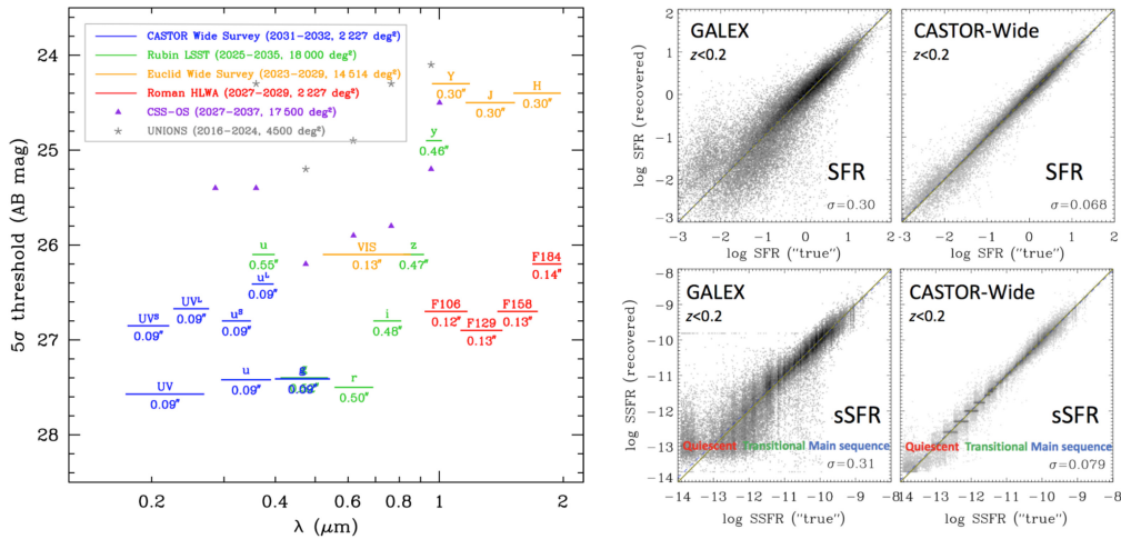
Fig. 9 (Left) Depths of wide-field UV/optical/IR imaging surveys plotted as a function of wavelength. Results are shown for several surveys: UNIONS, 23 LSST, 24 Euclid-Wide, 25 Roman-HLWA, 26 CSS-OS, 27 and CASTOR Wide. Note that CASTOR Wide targets the same footprint as the Roman HLWA survey. The labels under each filter indicate the survey’s approximate image quality (i.e., EE50 radius). (Right) Predicted improvements in the determination of SFR (upper panels) and specific SFR (lower panels) from the CASTOR Wide Survey (right panels) compared with the GALEX Medium-Deep Survey (left panels). The gains are most dramatic for quenching galaxies located in the transitional zone (i.e., the Green Valley).
