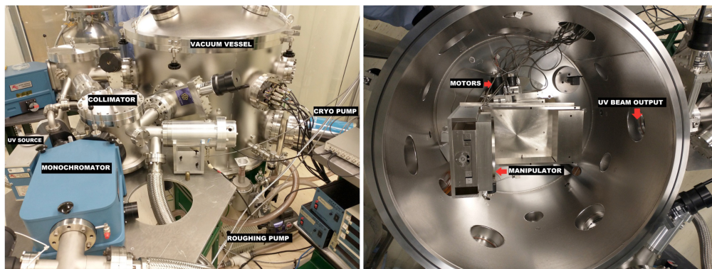
Fig. 20 (Left) View of the exterior hardware. (Right) Manipulator mounted inside of the vacuum vessel.
