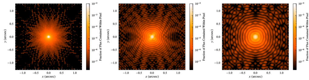
Fig. 6 Point spread functions (PSFs) at the field center in each of CASTOR's UV, u , and g channels (left to right). 17
