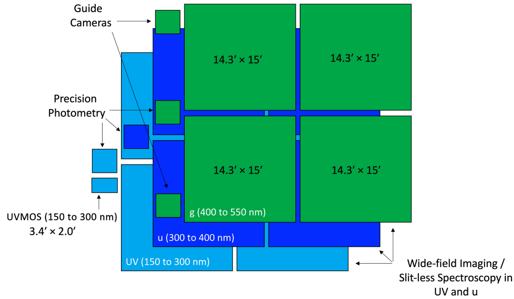
Fig. 5 Schematic view of CASTOR's instrument suite. Simultaneous wide-field imaging in the UV, u , and g passbands is enabled by dichroics that divide the incoming light into three channels covering the 0.15 to 0.55 \mu\text{m} range. A deployable grism provides low-resolution ( 300 \lesssim R \lesssim 420 ) slit-less spectroscopy over the full imaging field, in the UV and u channels. Each of CASTOR's three focal plane arrays (FPAs) is accompanied by a dedicated CMOS detector for high-precision photometric measurements of transiting exoplanets. Low-medium resolution long-slit and multi-slit spectroscopy is possible using a UVMOS instrument that observes an adjacent field. Two CMOS devices in the g -band channel provide spacecraft guiding.
