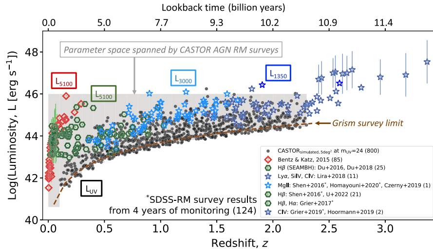
Fig. 11 Luminosity-redshift parameter space spanned by CASTOR (light gray area) compared with all previous studies (colored symbols). CASTOR will be able to probe uniformly a unique region in the phase space of redshift and luminosity (black circles showing a simulated sample in 5 deg 2 ) as well as galaxy-host properties to study how black holes grow and how they affect galaxy evolution over 10 billion years of cosmic time.
