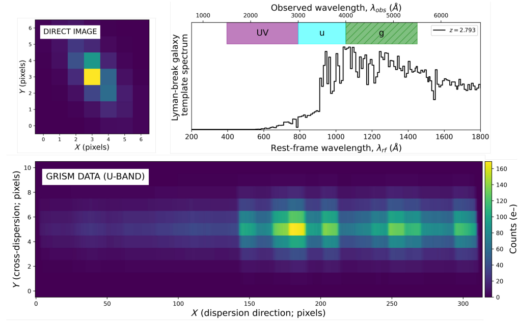
Fig. 18 Simulated CASTOR grism spectrum of a Lyman-break galaxy at z = 2.793 . The top left panel shows the simulated direct image of the source ( r_{\text{eff}} = 0.15'' , ellipticity of 0.55, Sérsic index n = 1.05 ) at CASTOR resolution. The top right panel shows the Lyman-break template used for the source SED. The shaded bands show the wavelength range of the CASTOR UV, u, and g channels (purple, cyan, and hatched green, respectively). Only the UV and u channels have grism capabilities. The bottom panel shows the noiseless electron counts of the simulated grism spectrum after 6 h of exposure for a u = 23.4 mag (AB) source. The grism tool also simulates the noise properties of the grism observations (including the sky background, read noise, and dark current) to produce SNR maps and derive exposure times.
