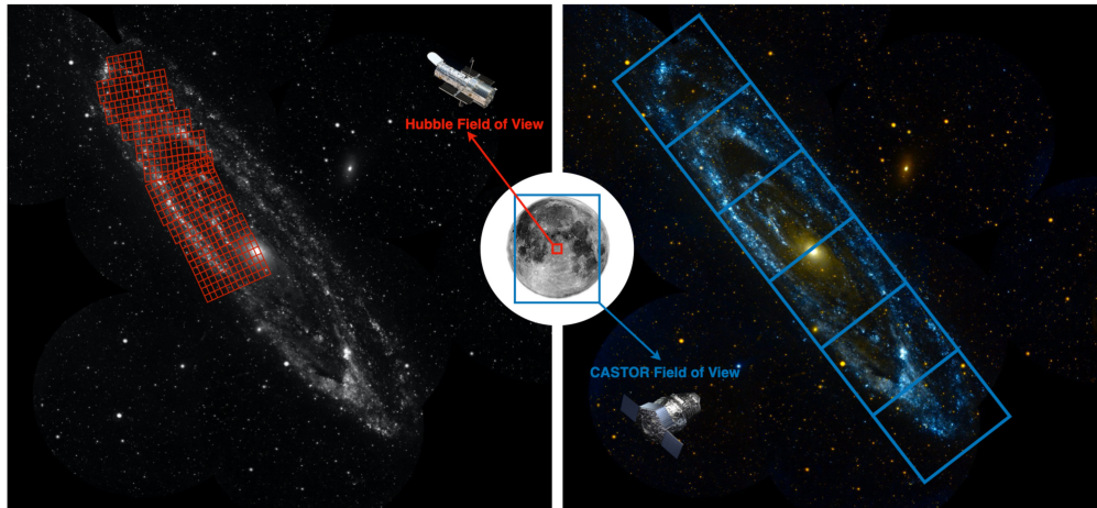
Fig. 1 Comparison of CASTOR’s field of view to that of the Hubble Space Telescope (HST) overlaid on an ultraviolet image from GALEX. 12 The figure on the left shows the distribution of HST fields from the Panchromatic Hubble Andromeda Treasury (PHAT)—one of the largest programs carried out with HST and the most comprehensive existing study of the Andromeda galaxy (M31). PHAT covered approximately a third of M31’s disk with 414 separate pointings, shown in the panel to the left, each of which was imaged six times in six different filters over a 40-day campaign. 13 The figure on the right shows how CASTOR could map the entirety of Andromeda’s disk in six pointings. The different HST and CASTOR fields are superimposed on the full moon, which is shown to scale at the center of the image.
