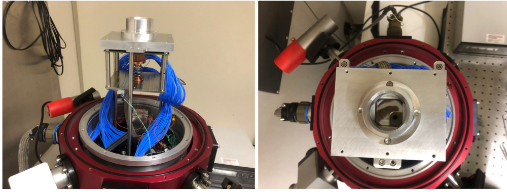
Fig. 21 Two views of the CIS120 detector and platen installed in the cryostat at NRC-HAA.
