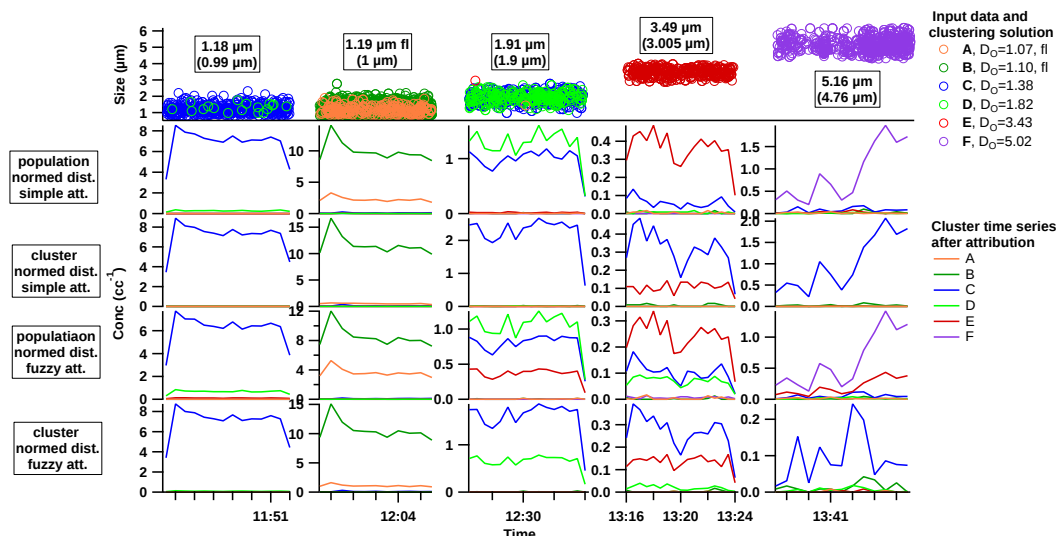
Fig. 5. Top plot shows the single-particle data input to the cluster analysis routine ( \sim 30\% of all the particles that were measured) coloured by their cluster, as defined in Table 3. Particle size and fluorescence for each retrieved cluster are detailed in the legend. Measured PSL optical diameters are detailed in boxes, with the actual PSL physical diameters in brackets. Below are cluster concentration time series after the remaining particles are attributed to the resolved clusters, using four different attribution algorithms, detailed on the left. The x-axis is discontinuous between the introduction of different PSLs. The y-axes are inconsistent between subplots.
