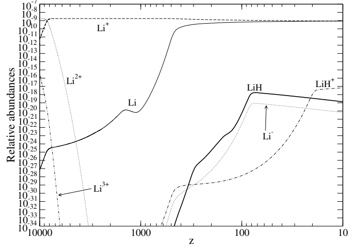
Fig. 8. Standard primordial chemistry of lithium species.
