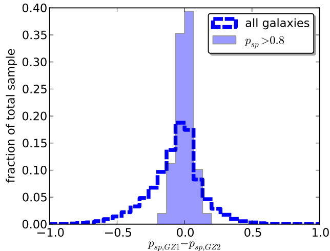
Figure 9. Comparison of the spiral feature vote fractions for objects in Galaxy Zoo 1 (GZ1) and Galaxy Zoo 2 (GZ2). The dashed line shows the difference between p_{\text{combined spiral}} for GZ1 and p_{\text{features or disk}} for GZ2 for the 240,140 galaxies in both samples. The filled histogram shows the same metric for the 57,994 galaxies classified as “clean” spirals in both GZ1 and GZ2.
