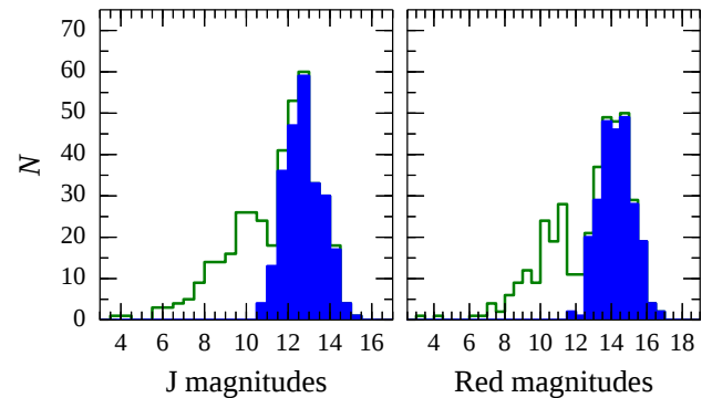
Figure 5. 2MASS J and red magnitudes distributions, for the 248 classical Be stars in the sample (solid blue) and for the previously known classical Be stars in the area (step histogram). Not all the previously known classical Be stars have 2MASS photometry so that only 152 are plotted in the left figure. Because fewer of the previously known classical Be stars in the area do not possess IPHAS r photometry either, we used USNO B1.0 photometry (Monet et al. 2003) as a close proxy.
