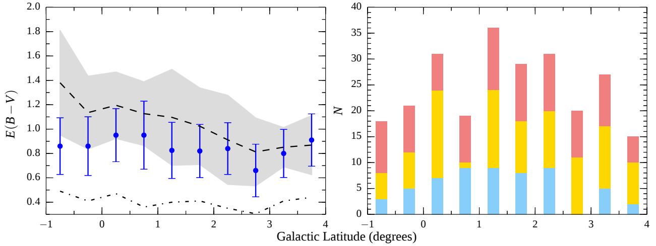
Figure 11. Left panel: mean interstellar reddening derived from the 247 classical Be stars in the catalogue on binning up into 0.5 deg strips parallel to the Galactic plane (marginalising over longitude). The error bars represent the 1- \sigma dispersion around the mean values. The upper dashed-curve and the shaded area trace the mean SFD98 values in each strip and the relative 1- \sigma dispersion, while the lower dot-dashed curve follows the mean RF09 values in each strip. Right panel: histogram bars representing the number of classical Be stars in each latitude bin, colour coded accordingly to the spectral classification (light blue: Early-B; gold: Mid-B; Late-B: pink).
