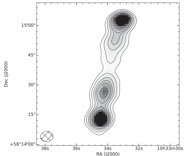
Figure 1. The bright source 3C 244.1 that falls in the LOFAR f.o.v. This source has a flux density of \sim 35 Jy beam ^{-1} and has been removed from the LOFAR images due to the artefacts it produced. The contour levels shown are 0.1, 0.25, 0.5, 0.75, 1.0, 1.5, 2.0, 3.0, 4.0 Jy. This image was made from 8-h observation with LOFAR using a bandwidth of 195 kHz at 150.7 MHz. The beam size is 5.3 \times 6.4 arcsec and the rms reached in this image is 2.6 mJy beam ^{-1} .
