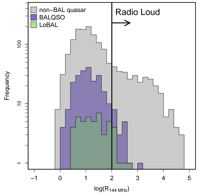
Fig. 7. Distributions of radio loudness of non-BAL quasars, BALQSOs, and LoBALs.
