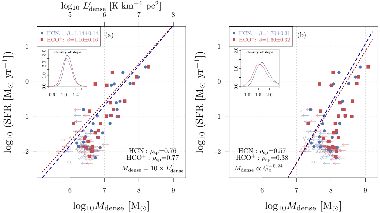
Figure 8. Dense-gas star-formation relationships (SFR versus M_{\text{dense}} ) using different conversion factors ( \alpha_{\text{dense}} ). M_{\text{dense}} in the left panel is calculated using a constant \alpha_{\text{dense}} , and the line luminosity L'_{\text{dense}} is shown as the original observable on the top x-axis in panel (a). M_{\text{dense}} in the right panel is calculated using a conversion factor \alpha_{\text{dense}}(G_0) , which is a function of the radiation field intensity G_0 . Because in panel (b) the \alpha_{\text{dense}} depends on G_0 we do not show the axis for L'_{\text{dense}} . The regression fits are plotted as blue and red dashed lines, matching the respective symbol colour of the HCN and HCO + data points. The slopes \beta are given by the Bayesian method for linear regression (Kelly 2007), accounting for uncertainties and upper limits. See the text for more details.
