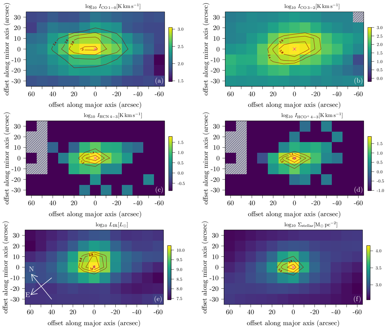
Figure 3. Maps of the different molecular-line emissions, infrared luminosity and stellar surface density. The units are given above each panel and all maps are logarithmic. Infrared luminosity is from Tan et al. (2018). Each pixel size is 10 arcsec or 171 pc. The hatched pixels are regions without available data, and the typical RMS of each map is shown as the lowest values. Contours start from 30% of the peaks, and the contour spacing is 0.2 dex. The magenta cross marks the galactic centre. Note that these images are rotated (see Fig. 1) to align with the major axis of NGC 253.
