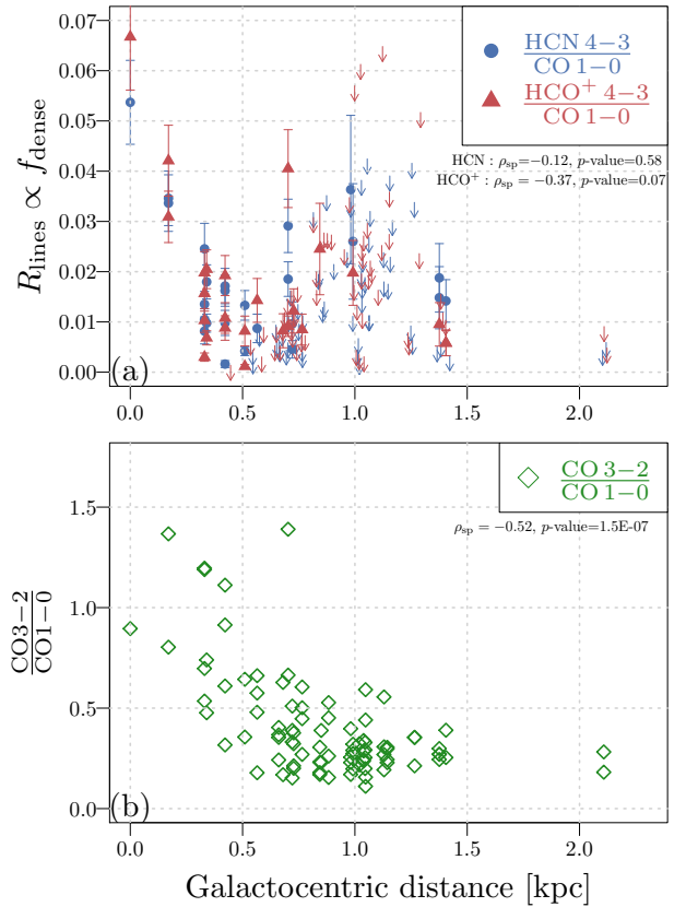
Figure 6. upper panel: Radial distribution of dense-gas fraction ( f_{\text{dense}} ) traced by the integrated-intensity ratios R_{\text{HCN}} = \text{HCN 4-3}/\text{CO 1-0} and R_{\text{HCO}^+} = \text{HCO}^+ \text{ 4-3}/\text{CO 1-0} . Arrows denote the upper limits of f_{\text{dense}} . bottom panel: Radial distribution of the ratio R_{31} between the two CO transitions.
