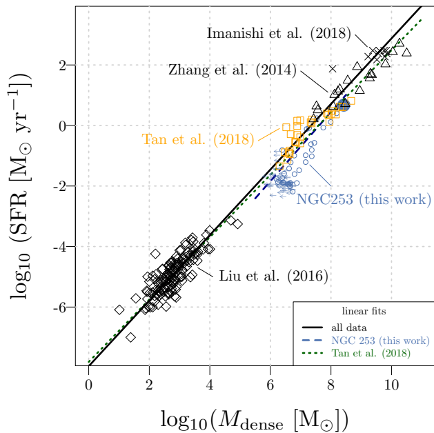
Figure 9. Dense-gas star-formation relationships (SFR versus M_{\text{dense}} ) for all HCN 4-3 samples compiled in this work. The filled circle is the sum value of the central \sim 0.9 kpc of NGC 253. The black solid line is a linear fit (in logarithmic scale) for all data ( \beta = 1.08 \pm 0.01 ). The blue dashed line is a fit for NGC 253 data from Fig. 8a ( \beta = 1.13 \pm 0.14 ). The dotted line is the fit ( \beta = 1.03 \pm 0.01 ) from Tan et al. (2018).
