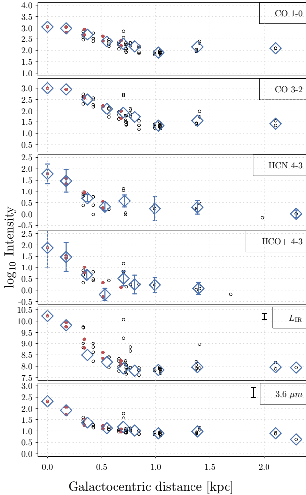
Figure 5. Radial distributions of different tracers used in this paper. The circles denote a data point extracted from each pixel in the final 13 \times 7 positions (Fig. A1), and the red filled circles indicate pixels situated on the major axis. Blue diamonds denote the mean values within each 0.17-kpc radial bin. The units are L_{\odot} for L_{\text{IR}} , \text{MJy sr}^{-1} for 3.6 \mu\text{m} , and \text{K km s}^{-1} for the molecular lines. The measurement errors of most individual data points are typically < 0.1 dex. For CO lines the uncertainty is dominated by the flux calibration (10 per cent). For HCN 4-3 and \text{HCO}^+ 4-3 the uncertainty of the binning data points is calculated based on the error from the individual pixels (see Section 3.3). For L_{\text{IR}} , the uncertainty is 30 per cent at most (Tan et al. 2018). For 3.6 \mu\text{m} , the uncertainty is considered to be \sim 50 per cent. For the last two panels we denote the typical error bar in the upper right corner.
