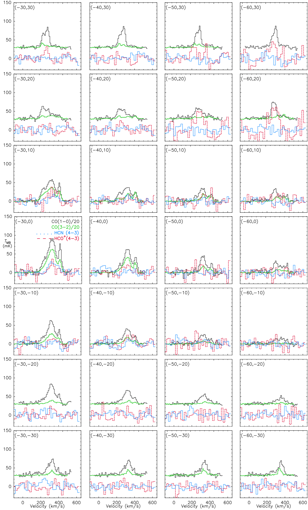
Figure A1 – continued Spectra of CO 1-0 (black), CO 3-2 (green), HCN 4-3 (blue) and HCO + 4-3 (red) emission in the central ~ 1 kpc region of NGC 253.
