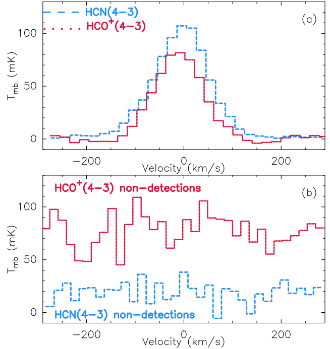
Figure 2. top panel: averaged spectrum of the central 5×3 pixels (~ 0.9 kpc along the major axis). bottom panel: averaged spectrum stacked from all the non-detections, with their velocities corrected according to the CO 3-2 line centre. The spectrum of HCO + 4-3 is shifted by 4 mK for clarity.
