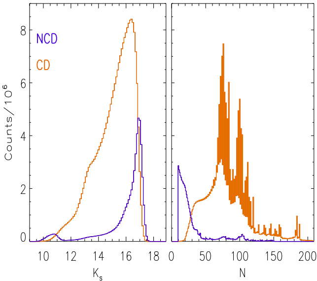
Figure 1. Histograms of K_s magnitude and number of measurements ( N ) for the VVV initial sample. The results for both NCD (blue lines) and CD (orange lines) are shown.
