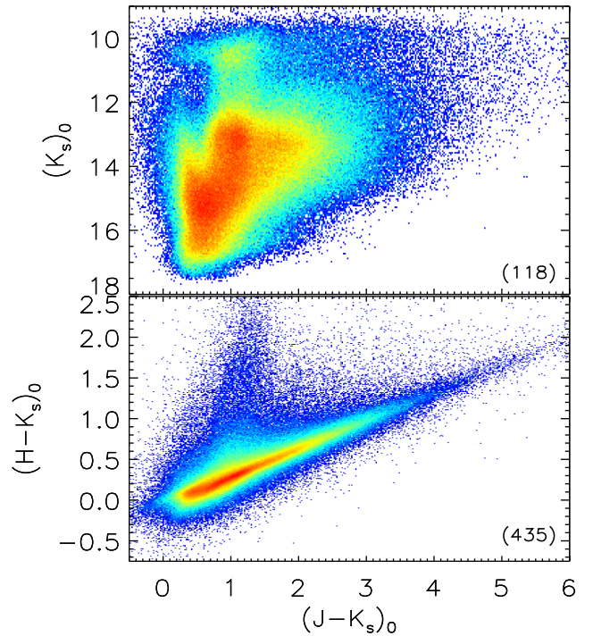
Figure 13. (J - K_s)_0 versus (K_s)_0 colour-magnitude diagram (upper panel) and (H - K_s)_0 versus (J - K_s)_0 colour-colour diagram (lower panel). The higher number of sources per pixel is shown in the right corner in each diagram. We should probably note that the brightest sources with K_s < 11 mag are saturated.
