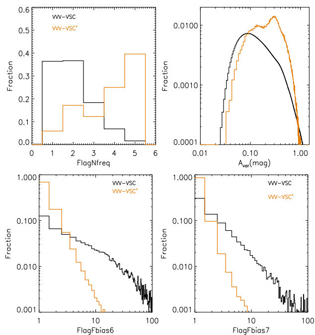
Figure 10. Histogram of FlagNfreq (upper left-hand panel), and A_{\text{VAR}} (upper right-hand panel), FlagFbias6 (lower left-hand panel), and FlagFbias7 (lower right-hand panel) for VVV-CVSC (black lines) and crossmatched sources having matched periods VVV-CVSC* (orange lines).
